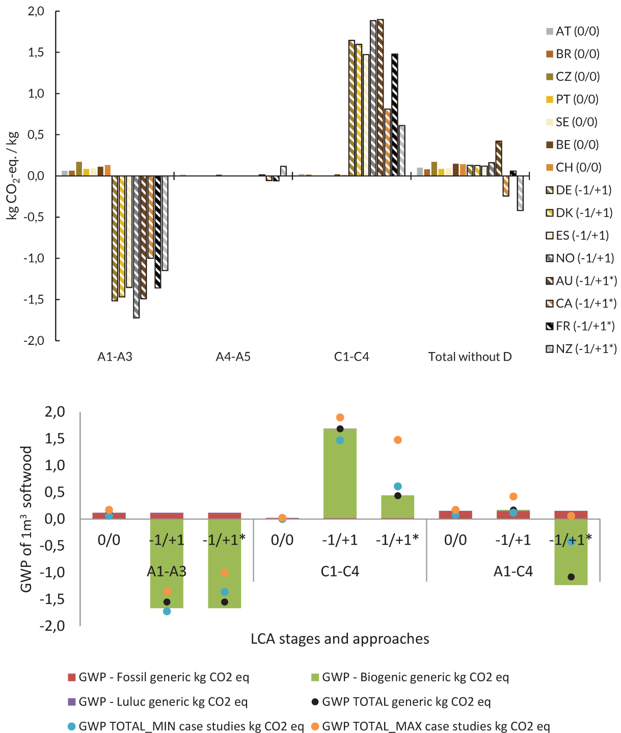
Figure 6: a) Greenhouse gas emissions in kg CO 2 -eq per kg solid softwood as assessed by the different countries and grouped according to the 0/0 and -1/+1 approaches, b) GWP of 1 m 3 planed, dried (MC=20%) softwood beam (density (wet) = 465 kg/m 3 , carbon content 0.494 kg/kg dry wood) (The modules A4-A5 and D are intentionally removed for clarity).
