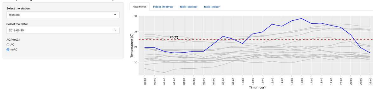
Figure 1. Screenshot from the RShiny app, which shows a comparison of indoor (gray lines) and outdoor (blue line) temperatures for non-air conditioned houses in the Montreal/St. Hubert weather station region on June 30, 2018.
