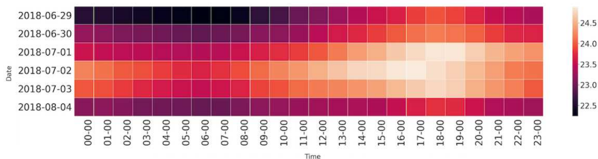
Figure 4. Average indoor temperatures for 47 households on heat wave days over time.
