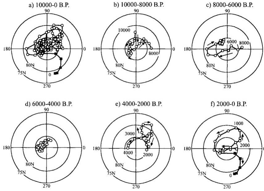
Figure 2.9 – (a) Location of the north geomagnetic pole for the last 10,000 years. (b)-(f) Geomagnetic pole positions for each 2000 year intervals. The dots represent the pole positions at 100 year intervals. From McElhinny and McFadden (2000).
