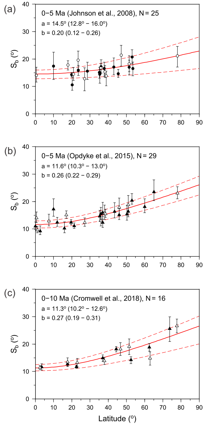
Figure 2.12 – VGP dispersion ( S_B ) as a function of latitude for three datasets: (a) 0-5 Ma (Johnson et al., 2008), (b) 0-5 Ma (Opdyke et al., 2015), and 0-10 Ma (Cromwell et al., 2018). The red line is the Model G curve with its 95% confidence intervals (dashed lines). N is the number of data used to fit the Model G (McFadden et al., 1988). VGP = virtual geomagnetic pole. Modified from Doubrovine et al. (2019).
