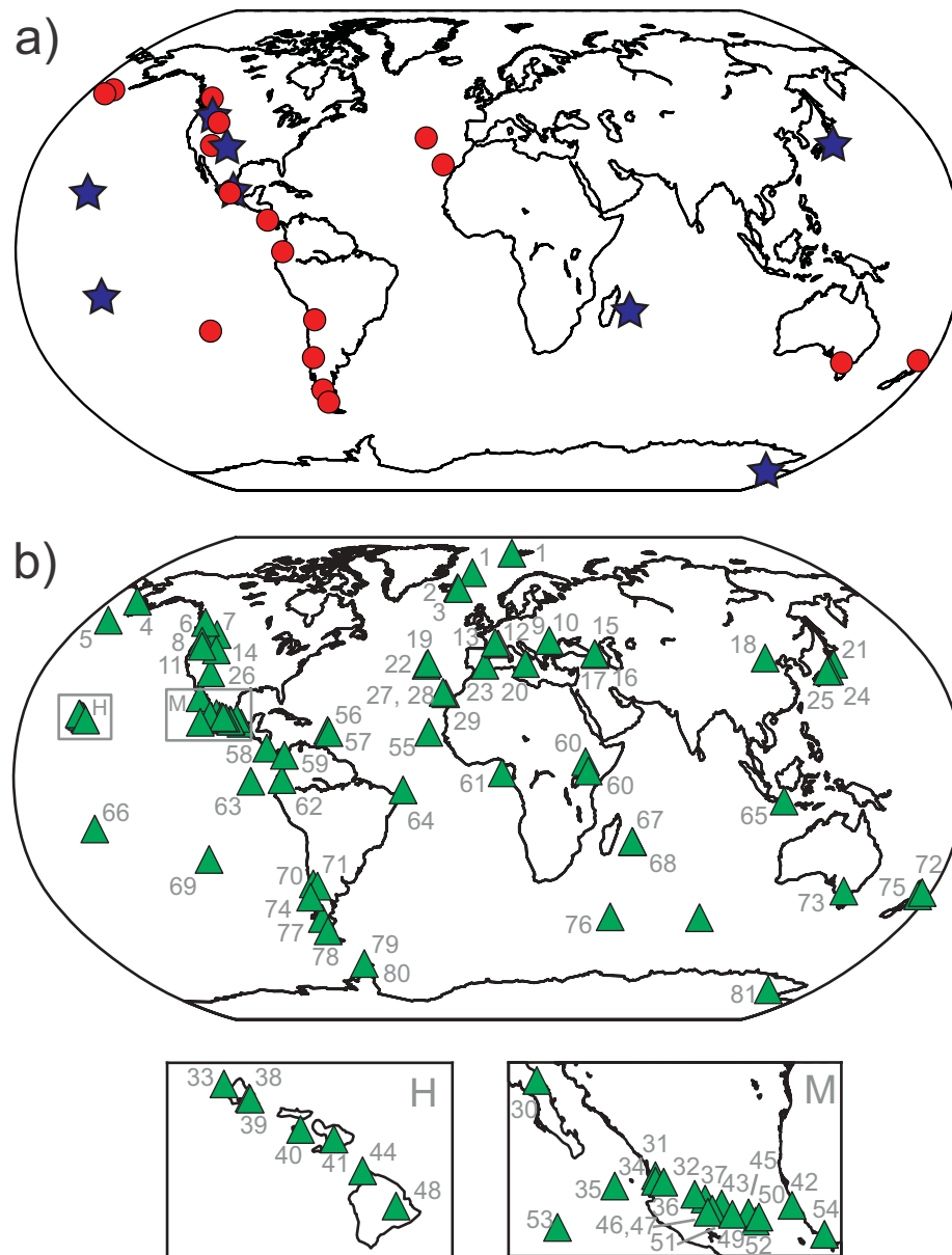
Figure 2.8 – Map with the location of paleomagnetic sites. (a) Database for the 0-5 Ma interval suggested by Johnson et al. (2008). The red circles (blue stars) indicate the locations of selected paleomagnetic studies (regional compilations). (b) Study locations (green triangles) from PSV10 dataset. Numbers correspond to the references reported in Table 2 of Cromwell et al. (2018). Modified from Cromwell et al. (2018).
