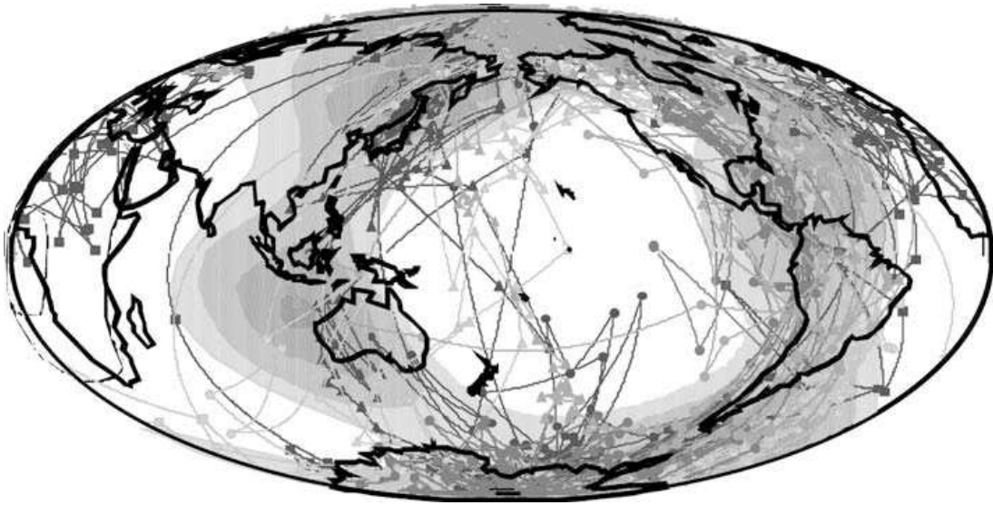
Figure 2.7 – Map showing the two preferred longitudinal sectors for transitional VGPs (black dots). The gray shaded areas indicate the high-velocity regions of seismic waves in the lower mantle. From Laj et al. (1991).
