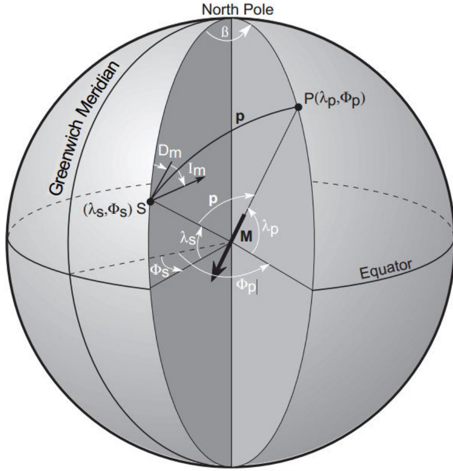
Figure 2.4 – Schematic of the position of a paleomagnetic pole P(\lambda_p, \phi_p) calculated from site location at S(\lambda_s, \phi_s) and mean magnetic direction ( I_m, D_m ). \mathbf{M} represents the geocentric magnetic dipole, p is the paleocolatitude, and \beta refers the longitudinal difference between pole and site. From Butler (1998).
