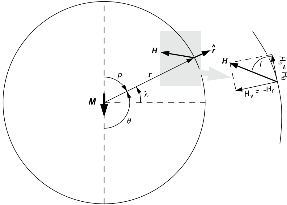
Figure A.1 – Representation of the geocentric axial dipole. The magnetic dipole moment \mathbf{M} is represented by the large arrow. The parameters \theta, p, \lambda, r are the polar angle, magnetic colatitude, geographic latitude and radial distance from the magnetic dipole, respectively. \mathbf{H} is the magnetic field yielded by the dipole, \hat{\mathbf{r}} is the unit vector in radial direction r . The gray shaded area shows the vector \mathbf{H} that can be divided into vertical ( H_v = -H_r ) and horizontal ( H_h = H_\theta ) components. From Butler (1998).
