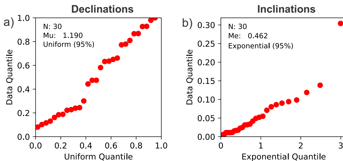
Figure E.7 – Quantile-quantile plots. (a) Declination data as a function of uniform distribution. (b) Inclination data as a function of exponential distribution.
