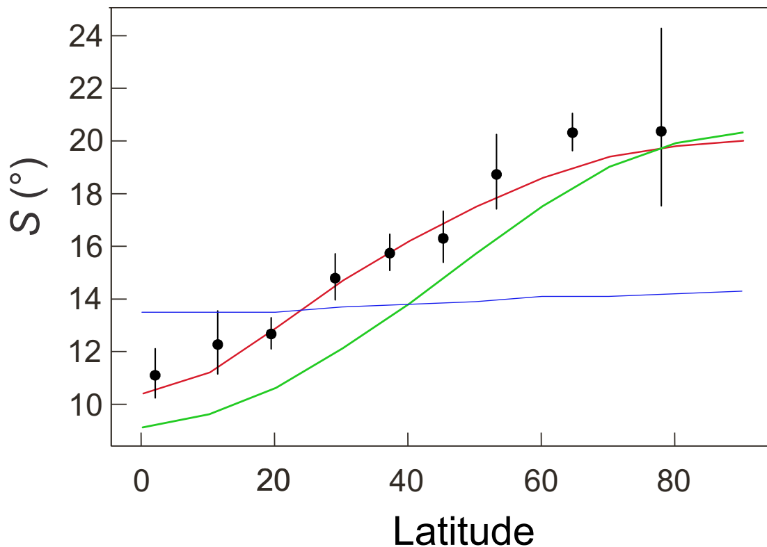
Figure 2.13 – VGP dispersion ( S ) as a function of latitude for MM97 dataset (McElhinny & McFadden, 1997) represented by black circles. Also shown are VGP dispersions predicted for three GGP models: CP88 (blue curve) of Constable and Parker (1988), CJ98 (green curve) of Constable and Johnson (1999), and TK03.GAD (red curve) of Tauxe and Kent (2004). Modified from Tauxe and Kent (2004).
