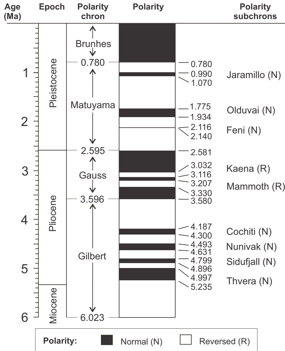
Figure 2.6 – Geomagnetic polarity time scale for the 0-6 Ma interval. Modified from Ogg (2020).
