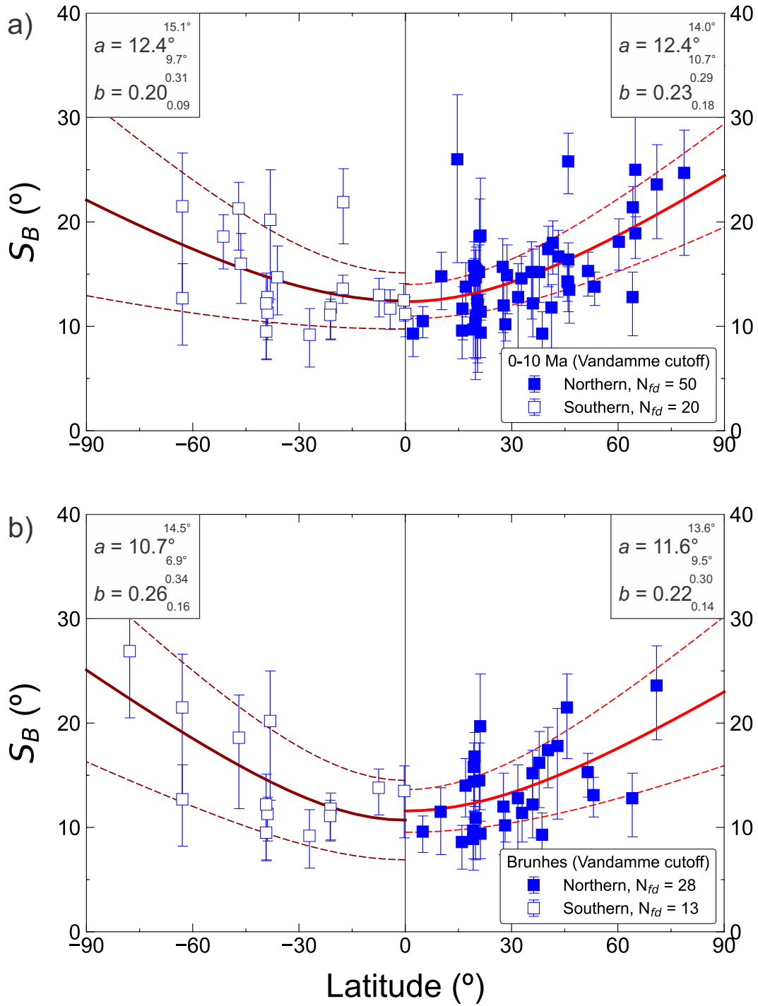
Figure 3.6 – VGP dispersion ( S_B ) as a function of latitude for (a) the 0-10 Ma interval, and (b) Brunhes chron applying the Vandamme (1994) cutoff. Light (dark) red lines represent the Model G curve fitted to northern (southern) hemisphere data, with its 95% confidence intervals (dashed lines).
