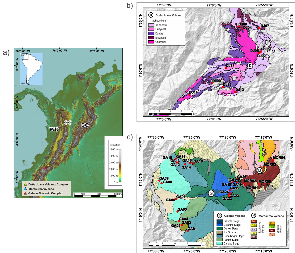
Figure 4.1 – (a) Topographic map of Colombia (WC: Western Cordillera; CC: Central Cordillera; EC: Eastern Cordillera) with the location of the three studied volcanic systems. Geologic maps of (b) Doña Juana Volcanic Complex, and (c) Morasurco Volcano and Galeras Volcanic Complex. Red circles indicate paleomagnetic site locations. Modified from Pardo et al. (2019), Trujillo et al. (2010), and Calvache et al. (1997).
