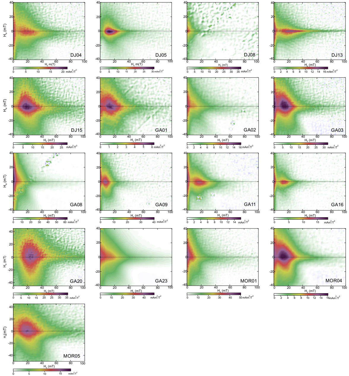
Figure E.4 – Examples of FORC diagrams. Details of magnetic domain structures are summarized in Table E.1
