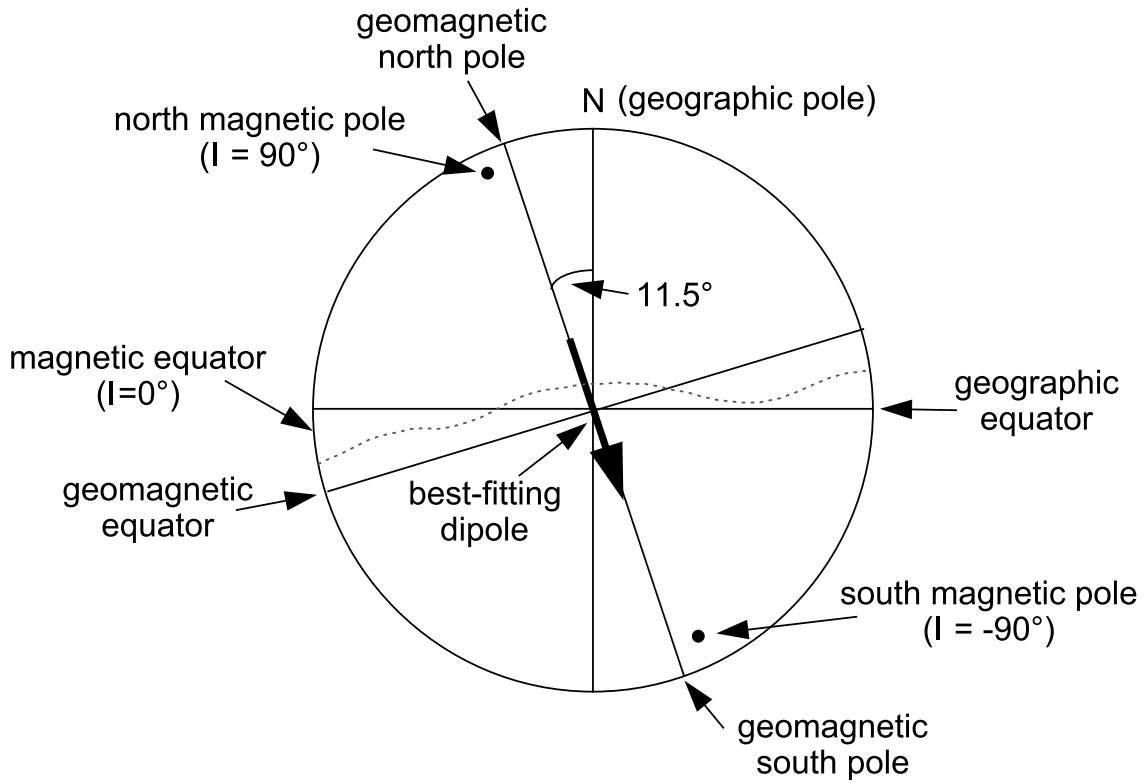
Figure 2.2 – Inclined geocentric dipole indicating the (geo)magnetic poles and equators. Modified from Butler (1998).
