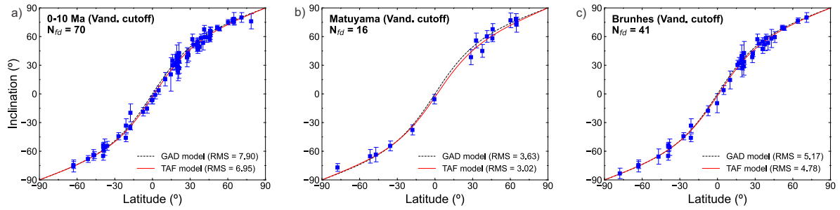
Figure 3.8 – Mean inclination as a function of latitude for (a) the 0-10 Ma interval, (b) Matuyama chron, and (c) Brunhes chron applying the Vandamme (1994) criterion. The uncertainties of the inclination data correspond to the 95% confidence cone ( \alpha_{95} ) of the mean direction. Black curves represent the expected GAD inclination. Red curves are the inclination predicted for TAF models proposed in this study (see Table 3.1). Vand. = Vandamme (1994); RMS = root mean square.
