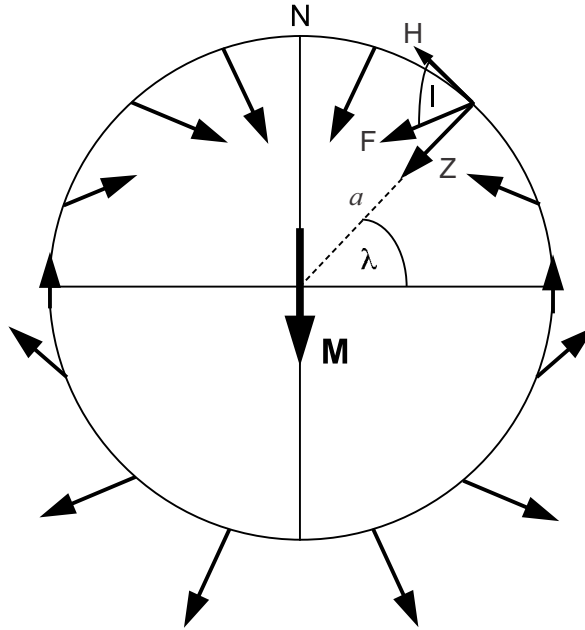
Figure 2.3 – Geomagnetic axial dipole model. Modified from Butler (1998).
