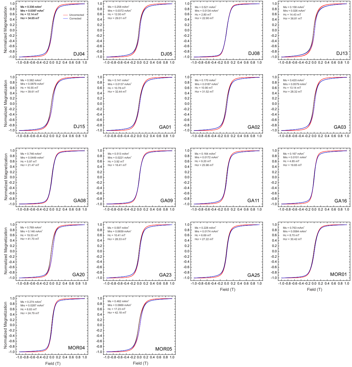
Figure E.2 – Examples of normalized hysteresis loops with their magnetic parameters (see Section 4.1.4.3 in the main article). Red (blue) curves show hysteresis loops with uncorrected (corrected) para- and diamagnetic contributions.
