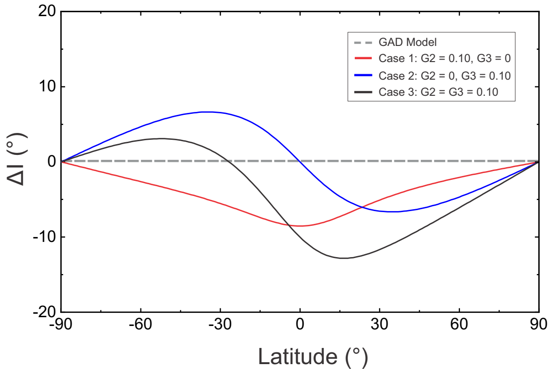
Figure 2.16 – Zonal models for the inclination anomaly ( \Delta I ) as a function of latitude.
