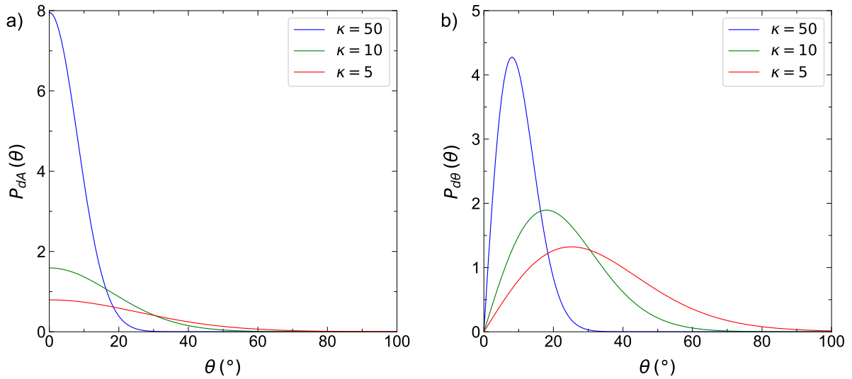
Figure B.1 – The Fisher distribution functions for \kappa = 5, 10 , and 50 . (a) P_{dA}(\theta) is the probability of a direction falling within a unit area dA at an angle \theta relative to the true mean. (b) P_{d\theta}(\theta) is the probability of finding a direction within an angular width d\theta between \theta and \theta + d\theta from the true mean. Modified from Butler (1998).
