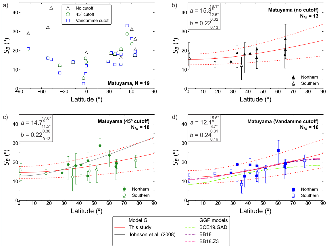
Figure 3.3 – VGP dispersion ( S_B ) as a function of latitude for the Matuyama reverse polarity chron. (a) S_B results with interhemispheric coverage defined using three VGP cutoff approaches. See Figure 3.2 caption for details. The gray line in (c) denotes the Model G curve fitted to the Matuyama data of Johnson et al. (2008).
