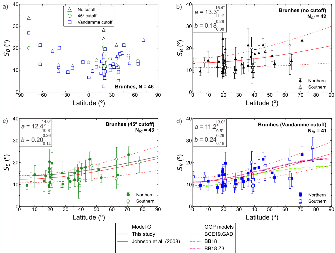
Figure 3.4 – VGP dispersion ( S_B ) as a function of latitude for the Brunhes normal polarity chron. (a) S_B results with interhemispheric coverage defined using three VGP cutoff approaches. See Figure 3.2 caption for details. The gray line in (c) denotes the Model G curve fitted to the Brunhes data of Johnson et al. (2008).
