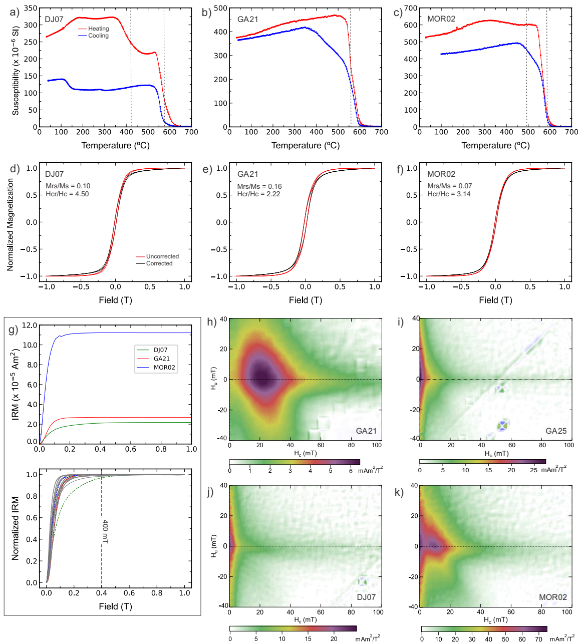
Figure 4.3 – Rock magnetic results for representative samples. (a-c) Thermomagnetic curves with heating (red curve) and cooling (blue curve) cycles. Dashed lines indicate the magnetic transition temperatures. (d-f) Normalized hysteresis loops, where red curves are not corrected for high field slopes. (g) IRM acquisition curves for 3 sites (top) and normalized IRM results for 21 sites (bottom). (h-k) FORC diagrams with magnetic domain structures for (h) vortex, (i-j) multidomain (MD), and (k) a mixture of vortex state and MD grains. IRM = isothermal remanent magnetization; FORC = first-order reversal curve.
