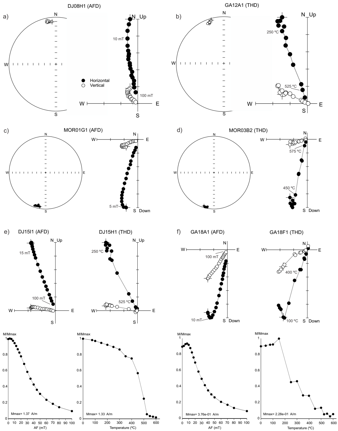
Figure 4.4 – Examples of demagnetization diagrams. Zijderveld diagrams and stereographic projections of NRM components obtained during (a and c) alternating field demagnetization (AFD) and (b and d) thermal demagnetization (THD). (e-f) Orthogonal projections of sister specimens using two demagnetization methods with demagnetization curves (below). Filled (open) circles correspond to vector components in the horizontal (vertical) plane for Zijderveld projections and upper (lower) hemisphere for stereographic projections. NRM = natural remanent magnetization.
