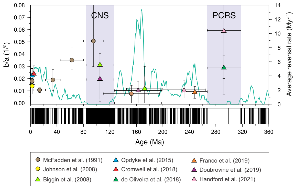
Figure 2.11 – Variations in b/a ratio from paleolecular variation studies covering Phanerozoic times, associated with the geomagnetic polarity time scale of Ogg (2020). Circles and triangles denote the best estimates for Model G parameters provided by studies applying a fixed ( 45^\circ or 40^\circ ) and Vandamme (1994) VGP cutoffs, respectively. The green curve represents the average reversal rate suggested by Doubrovine et al. (2019). The violet areas indicate the CNS (Cretaceous Normal Superchron) and PCRS (Permo-Carboniferous Reverse Superchron) intervals. VGP = virtual geomagnetic pole. Modified from Doubrovine et al. (2019).
