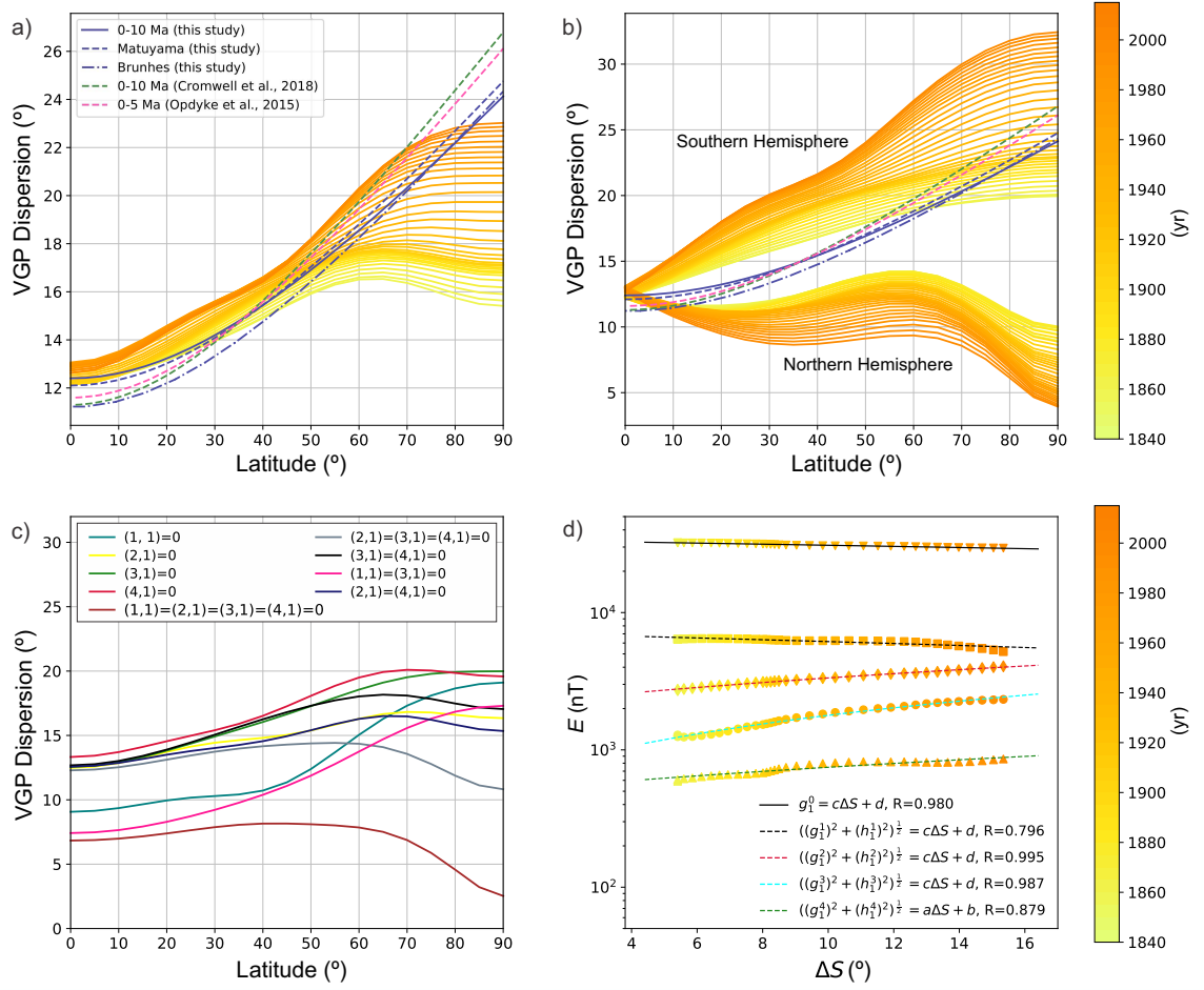
Figure 3.7 – Equivalent VGP dispersion as a function of latitude for the historical period from the COV-OBS field model (a) averaged over both hemispheres, (b) for the northern and southern hemispheres separately. (c) Equivalent VGP dispersion curves defined in terms of the Gauss coefficients filtered from the COV-OBS model for the 1965 epoch. (d) Average spherical harmonics energy as a function of interhemispheric variance ( \Delta S ) from historical VGP dispersions. Solid and dashed lines correspond to linear regressions fitted to \Delta S estimates defined for the axial dipole term ( g_1^0 ) and four non-zonal harmonic terms, respectively.
