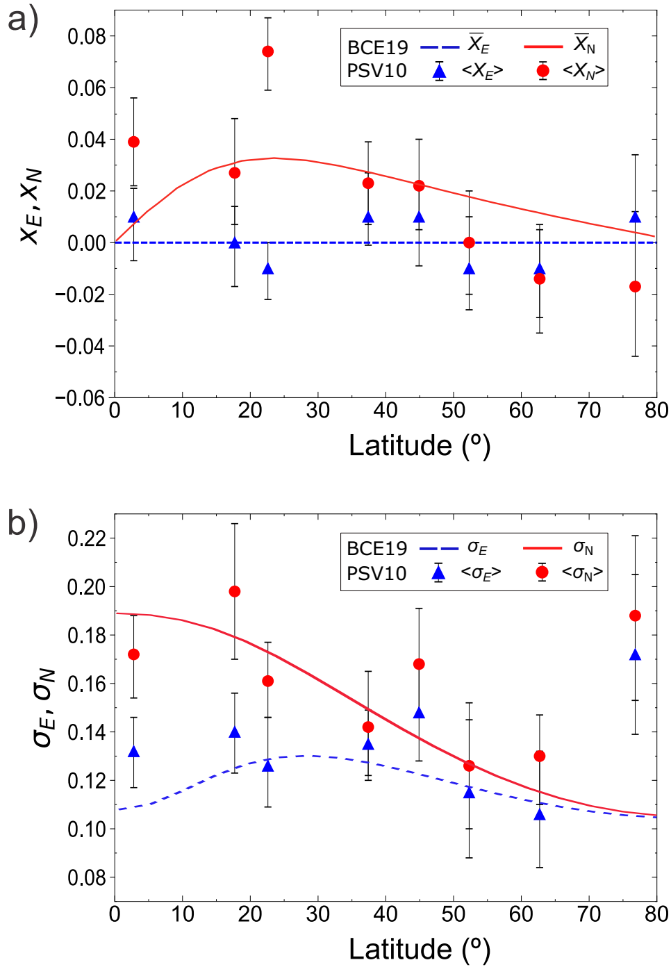
Figure 2.14 – Latitudinal distribution of directional measurements for PSV10 dataset (Cromwell et al., 2018). (a) Equal-area coordinates and (b) standard deviations along the axes north-south (east-west) are represented by red (blue) symbols. The curves are BCE19 model (Brandt et al., 2020) predictions. Modified from Brandt et al. (2020).
