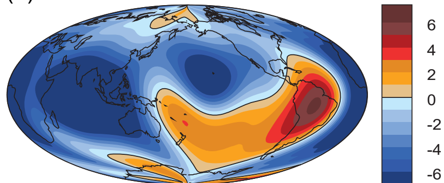
Figure 2.17 – Spatial variations of the inclination anomaly (in degrees) on the Earth's surface for the TAF models (a) LN3 and (b) LN1. Modified from Cromwell et al. (2018).
