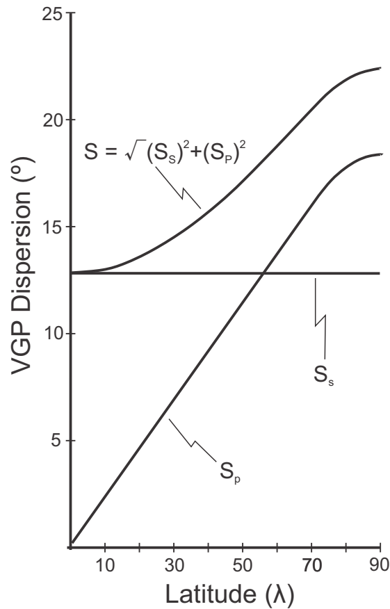
Figure 2.10 – Schematic representation of Model G. Modified from McFadden et al. (1991).
