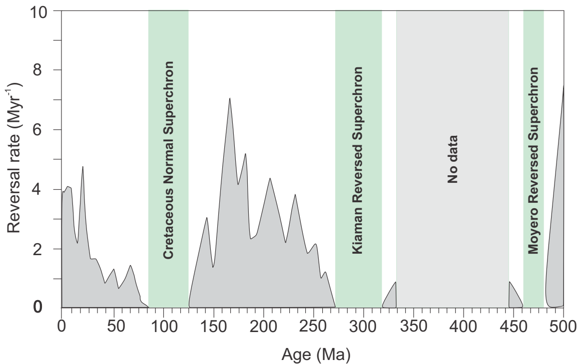
Figure 2.5 – Variations in geomagnetic reversal frequency for the last 500 Myr. Modified from Pavlov and Gallet (2005).
