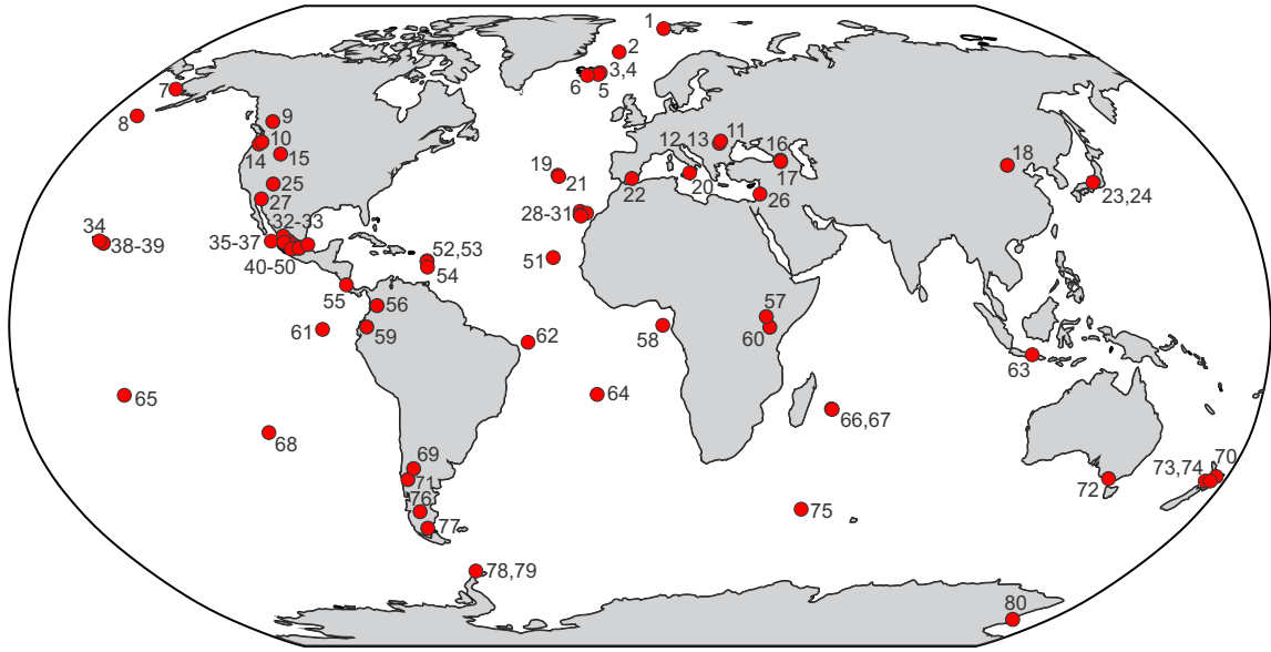
Figure 3.1 – Global distribution of selected paleodirectional data over the past 10 Myr. Numbers represent identification numbers reported in Table S1.
