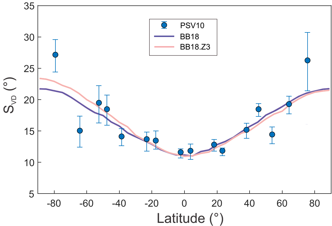
Figure 2.15 – Latitudinal variation of S_{VD} data for PSV10 dataset (Cromwell et al., 2018) are shown by blue circles. The pink and purple curves denote the BB18.Z3 and BB18 models (Bono et al., 2020) predictions, respectively. S_{VD} = VGP dispersion data filtered with Vandamme (1994) criterion. Modified from Bono et al. (2020).
