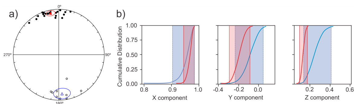
Figure E.6 – (a) Equal area projection of site-mean directions for normal (closed circles) and reverse (open circles) dataset. Red (blue) triangles represent the mean directions with their 95% confidence intervals for normal (reverse) polarity data. (b) Bootstrap reversal test defined by cumulative distributions of cartesian components for mean normal (red line) and mean reverse (blue line) directions. Red (blue) shaded areas are the 95% confidence regions for normal (reverse) modes.
