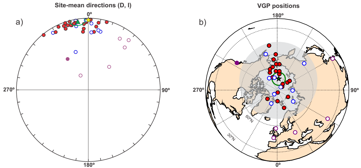
Figure 4.5 – Equal area projection of site-mean directions for the filtered dataset ( N = 30 sites). (a) Filled red (open blue) circles represent normal (antipodes of reversed) polarity directions. Green triangle represents the mean direction with its 95% confidence circle (green circle). The yellow star is the expected GAD direction. Purple circles indicate transitional data based on the Vandamme (1994) criterion and were not used for PSV and TAF analysis. (b) Polar stereographic map of VGP positions. Closed (open) circles correspond to normal (reversed) polarity site VGPs projected onto the Northern Hemisphere. The green star indicates the paleopole position with its 95% confidence circle (green circle). Data for transitional sites (purple circles) that were removed after applying the Vandamme (1994) cutoff ( 32.6^\circ ) are outside the transparent grey circle. GAD = geocentric axial dipole; VGP = virtual geomagnetic pole.
