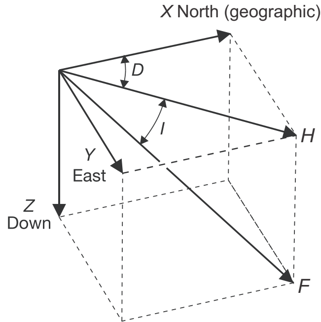
Figure 2.1 – Geomagnetic field components. The total intensity vector F is represented by three magnetic elements: X (northwards), Y (eastwards), and Z (vertical). H corresponds the horizontal component of F . D (declination) and I (inclination) define the magnetic direction. From McElhinny and McFadden (2000).
