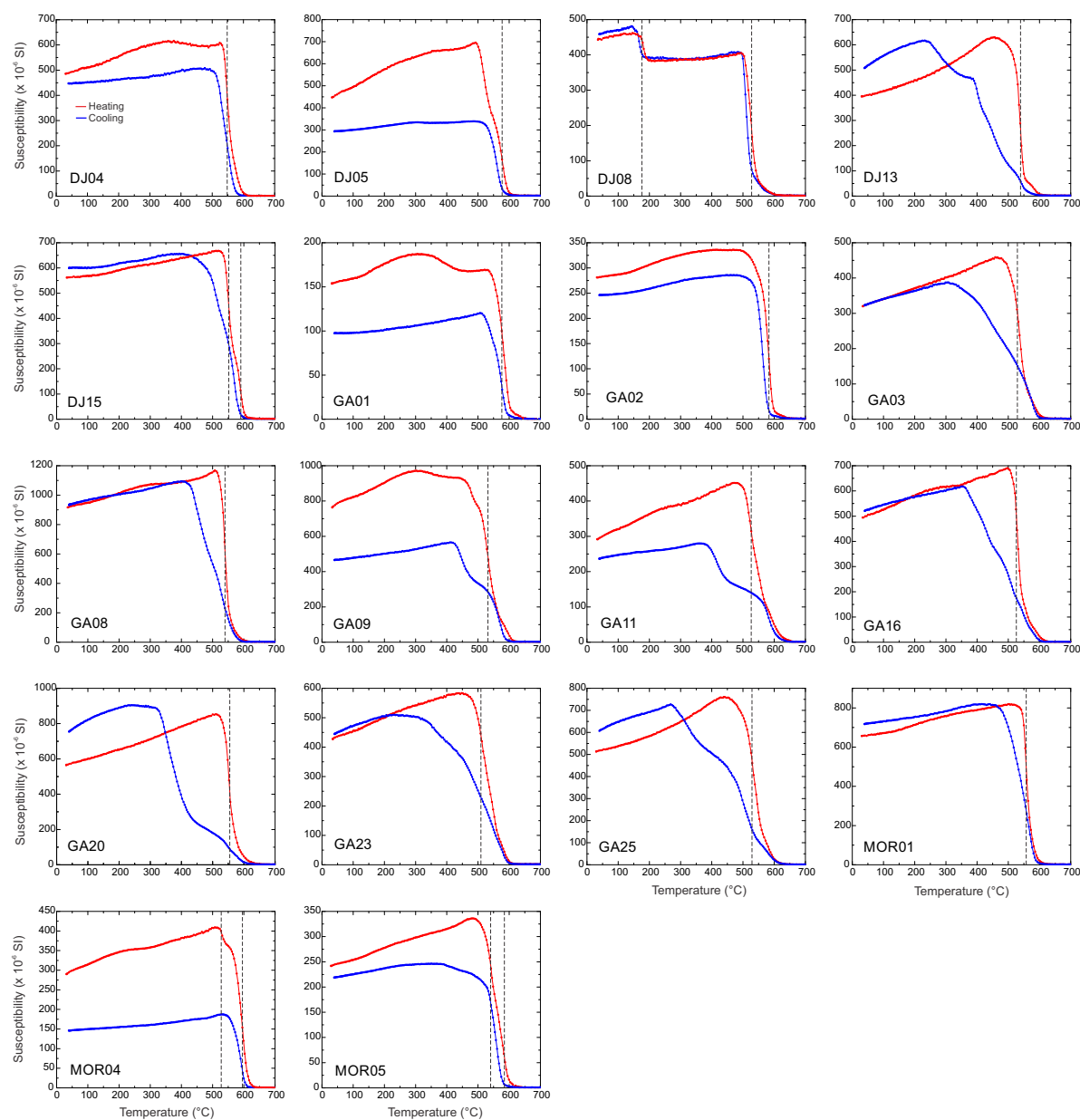
Figure E.1 – Examples of thermomagnetic curves during heating (red curve) and cooling (blue curve) cycles. Dashed lines indicate the Curie temperatures ( T_c ) summarized in Table E.1.
