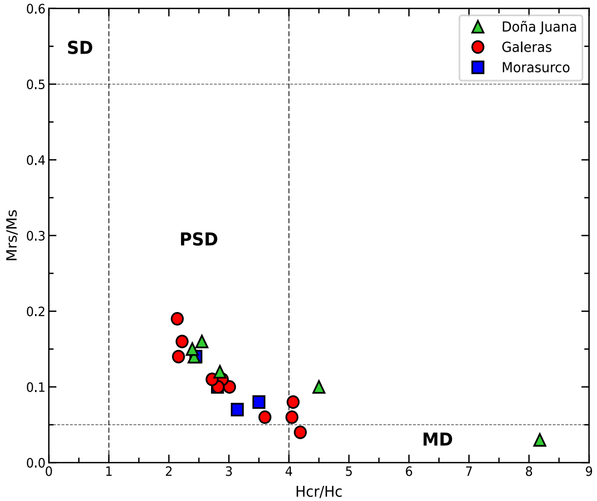
Figure E.3 – Day plot of representative samples (from 21 paleomagnetic sites). The estimates of hysteresis parameter ratios M_{rs}/M_s and H_{cr}/H_c are listed in Table E.1. SD = single domain; PSD = pseudo-single domain (or vortex state); MD = multidomain.
