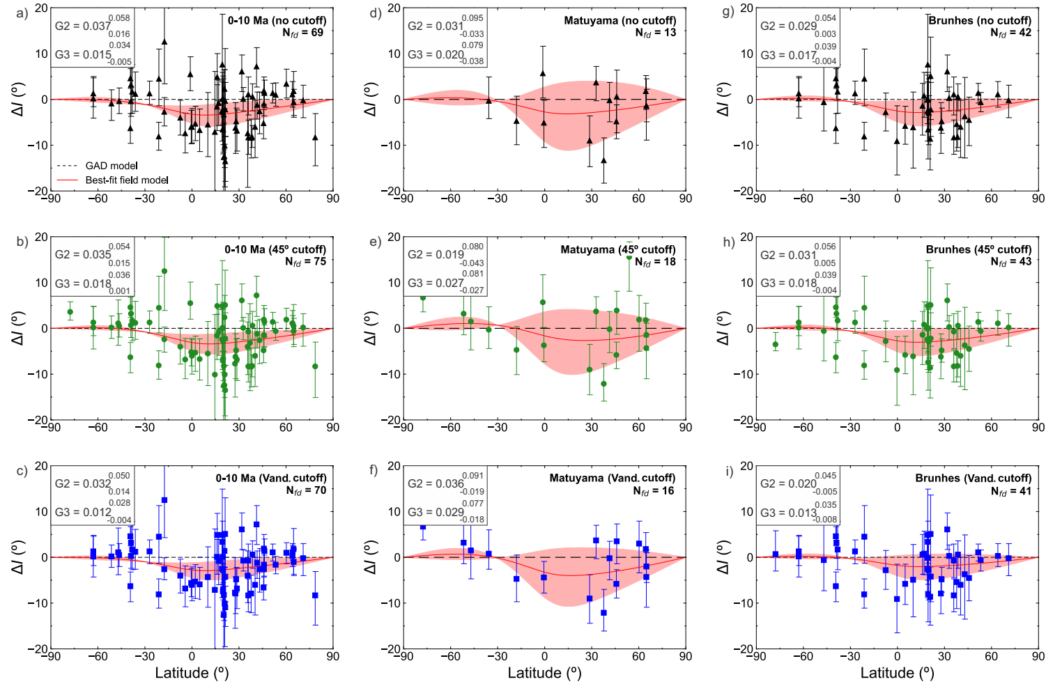
Figure 3.5 – Inclination anomaly ( \Delta I ) as a function of latitude defined using three VGP cutoff approaches. \Delta I estimates with 95% bootstrap confidence limits for (a-c) the 0-10 Ma interval, (d-f) Matuyama reverse chron, and (g-i) Brunhes normal chron. Red curves are the best-fit field model for each time period. Red-shaded areas represent the 95% confidence region associated with uncertainties for the zonal quadrupole ( G2 ) and octupole ( G3 ) terms. Each figure includes a GAD field model (black dashed line) at \Delta I = 0 . Vand. = Vandamme (1994).
