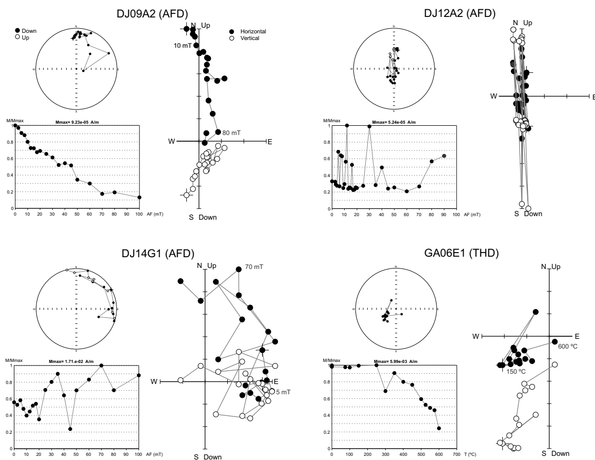
Figure E.5 – Examples of demagnetization diagrams for highly scattered data. Zijdeveld diagrams, stereographic projections, and demagnetization curves of NRM components for sites (a) DJ09, (b) DJ12, (c) DJ14, and (d) GA06. NRM = natural remanent magnetization.
