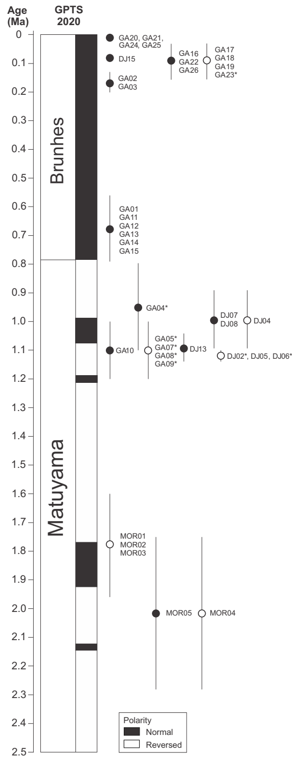
Figure 4.6 – Magnetic polarity of the paleomagnetic sites from this study compared to the geomagnetic polarity time scale 2020 (GPTS2020) of Ogg (2020). Black (white) circles denote normal (reversed) polarity. The age range attributed to the studied sites is represented by a vertical line supported by geochronological studies (see Table 4.1). *Transitional sites identified using the Vandamme (1994) criterion.
