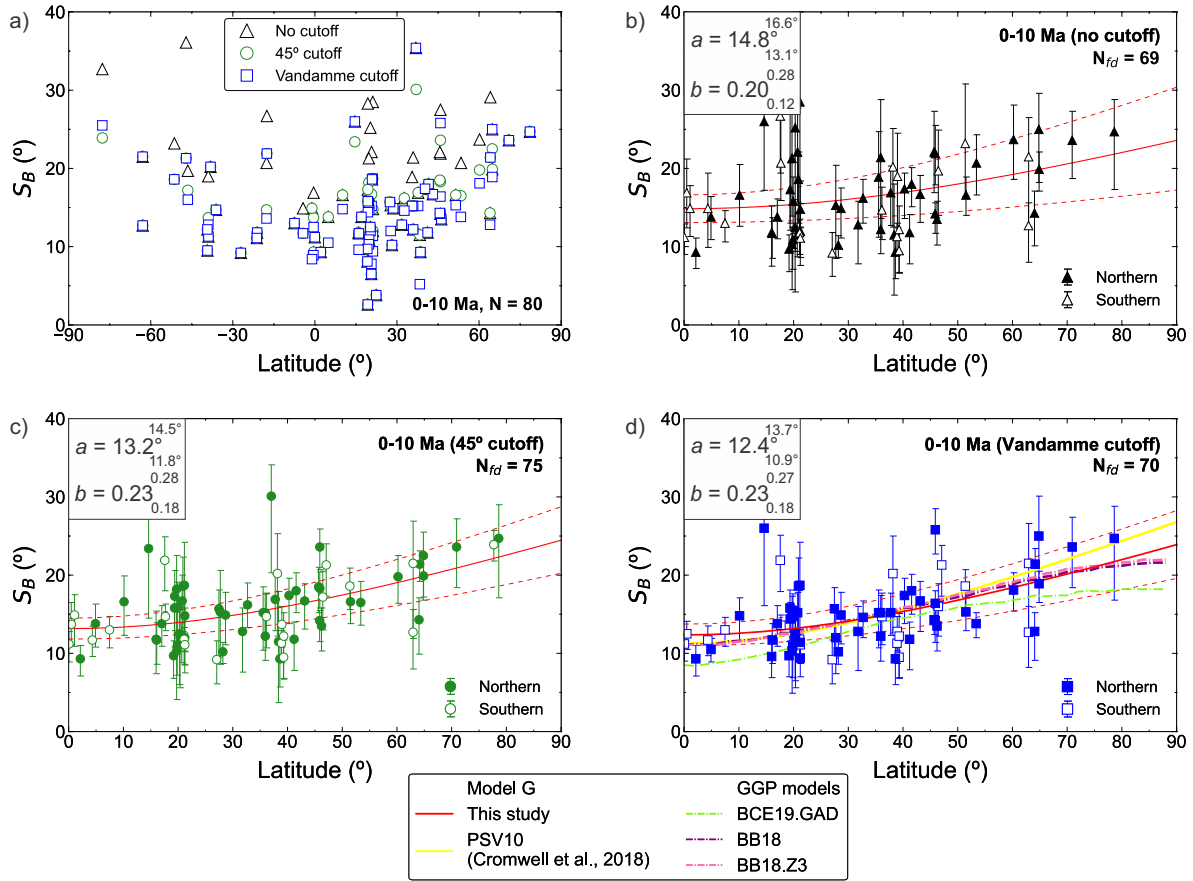
Figure 3.2 – VGP dispersion ( S_B ) as a function of latitude for (a) 0-10 Ma S_B results with interhemispheric coverage defined using three VGP cutoff approaches. (b-d) S_B estimates with 95% bootstrap confidence limits projected onto a single hemisphere. Closed (open) symbols correspond to data from the northern (southern) hemisphere. The best-fit Model G curves (McFadden et al., 1988) to S_B data are represented by red lines, associated with 95% confidence intervals (red dashed lines). (b) No cutoff applied, (c) 45° cutoff, and (d) Vandamme (1994) cutoff. In (d), the yellow line denotes the Model G curve fitted to the PSV10 data compilation (Cromwell et al., 2018). Also shown are VGP dispersions predicted for three GGP models: BCE19.GAD model of Brandt et al. (2020); light green dash-dot line; BB18 and BB18.Z3 models (Bono et al., 2020) purple and pink lines, respectively.
