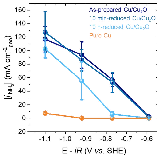
Figure A6. \text{NH}_3 partial current densities normalized by geometric areas for as-prepared, 10 min-reduced and 10 h-reduced \text{Cu}/\text{Cu}_2\text{O} (shades of blue) and pure Cu (orange). The results were obtained from 10 minutes of potentiostatic electrolysis with the catalyst as WE, graphite rod as CE and \text{Ag}/\text{AgCl} as RE, electrolyte containing 0.5 \text{ mol L}^{-1} \text{Na}_2\text{SO}_4 adding 0.05 \text{ mol L}^{-1} \text{NaNO}_3 in the catholyte.
