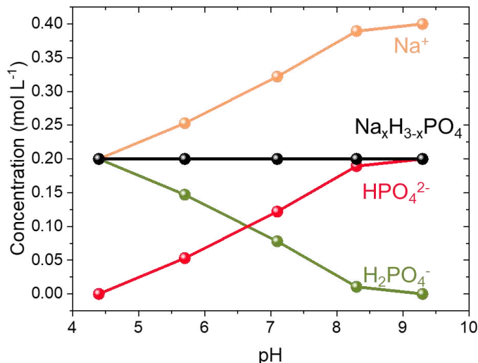
Figure 3.1. Ions' concentration and the solution pH of 0.2 \text{ mol L}^{-1} \text{ Na}_x\text{H}_{3-x}\text{PO}_4 (black line) electrolytes from pH 4.4 to 9.3.
