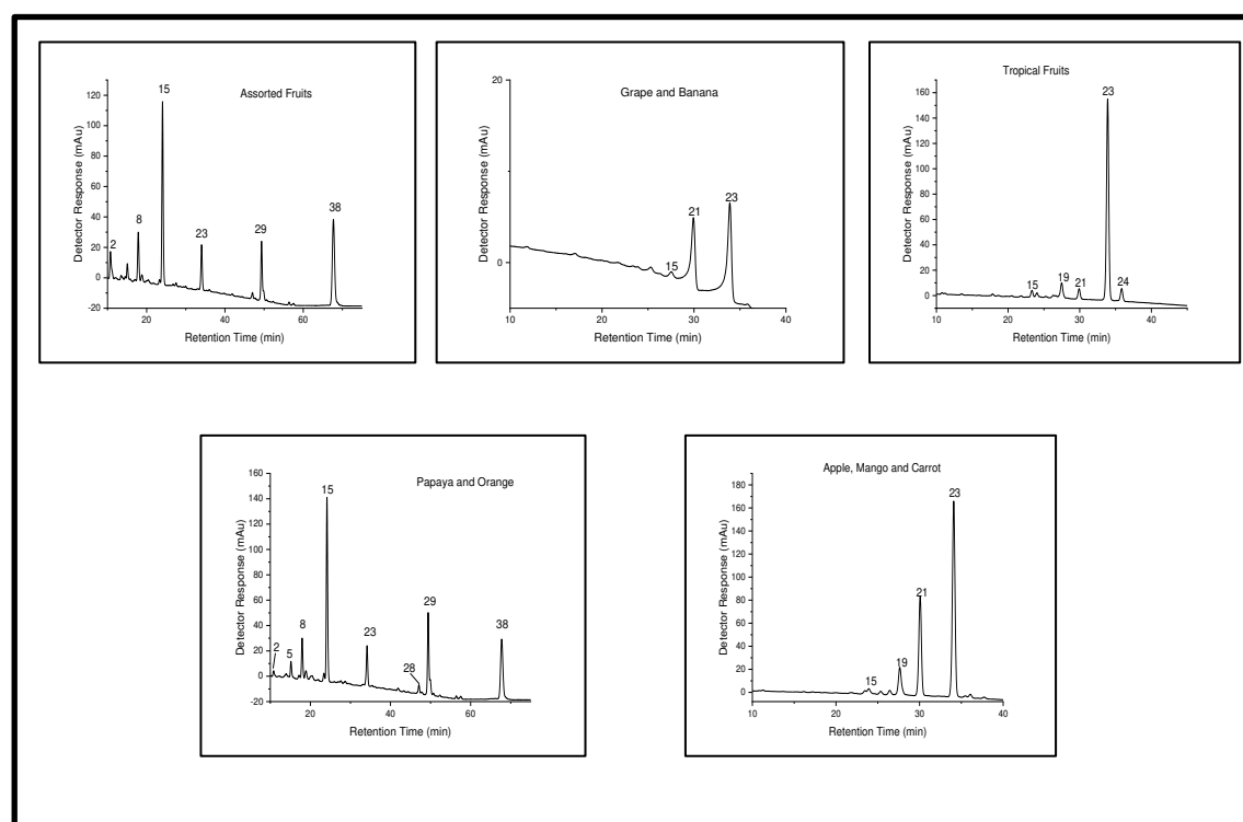
Figure 1 Chromatograms of carotenoids from homemade baby food, obtained by HPLC-DAD and processed at 450 nm. Peaks are numbered according to Table 7.
