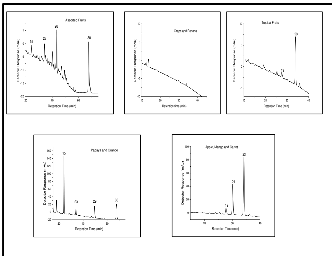
Figure 4 Chromatograms of carotenoids from digested homemade baby food, obtained by HPLC-DAD and processed at 450 nm. Peaks are numbered according to Table 7.
