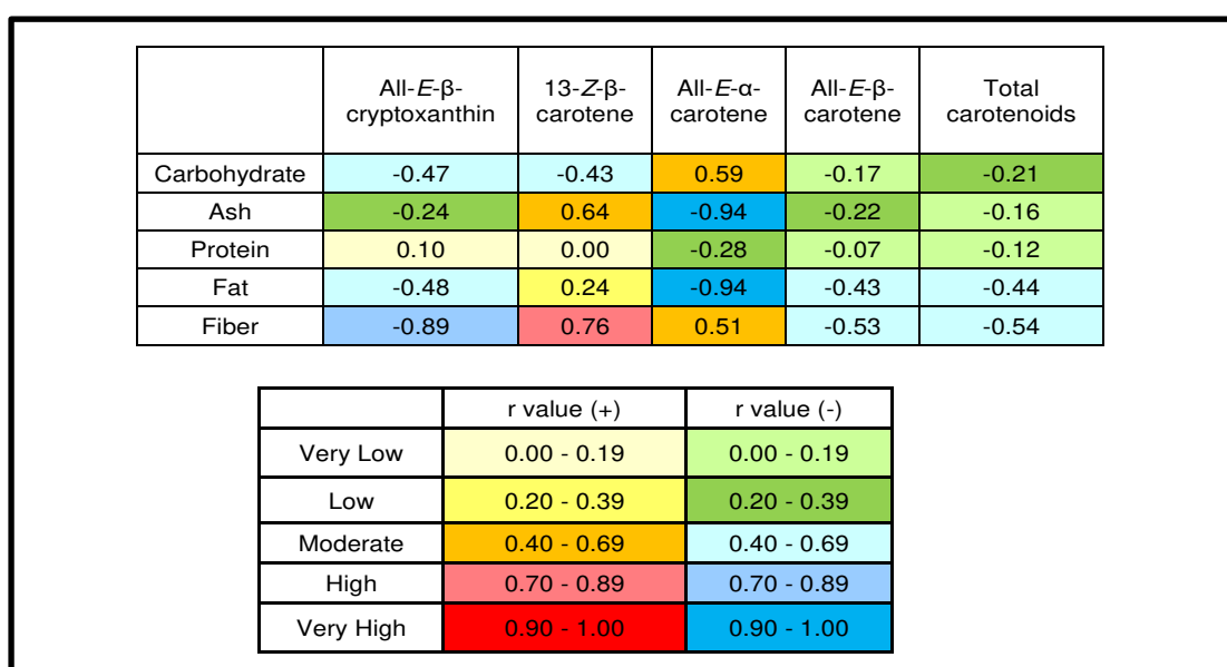
Figure 6 Pearson's correlation between individual and total carotenoids and proximate composition in homemade baby food. The r values are indicated according to the color legend ( p < 0.05\% ).
