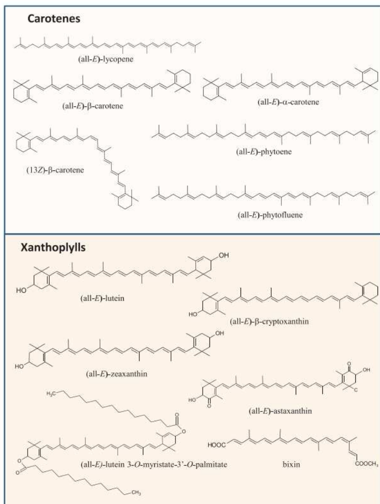
FIGURE 5.1 Molecular structures of carotenoids. Own authorship created by ACD/ChemSketch Freeware.
