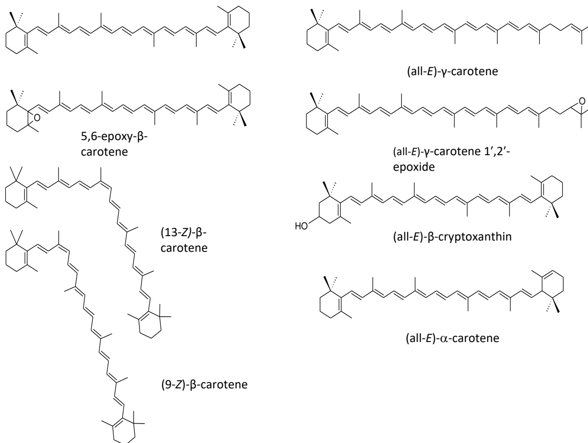
Fig. 1 Carotenoids with provitamin A activity. The central enzymatic cleavage of (all- E )-β-carotene can generate two retinol molecules, all other provitamin A carotenoids can only yield one molecule.
