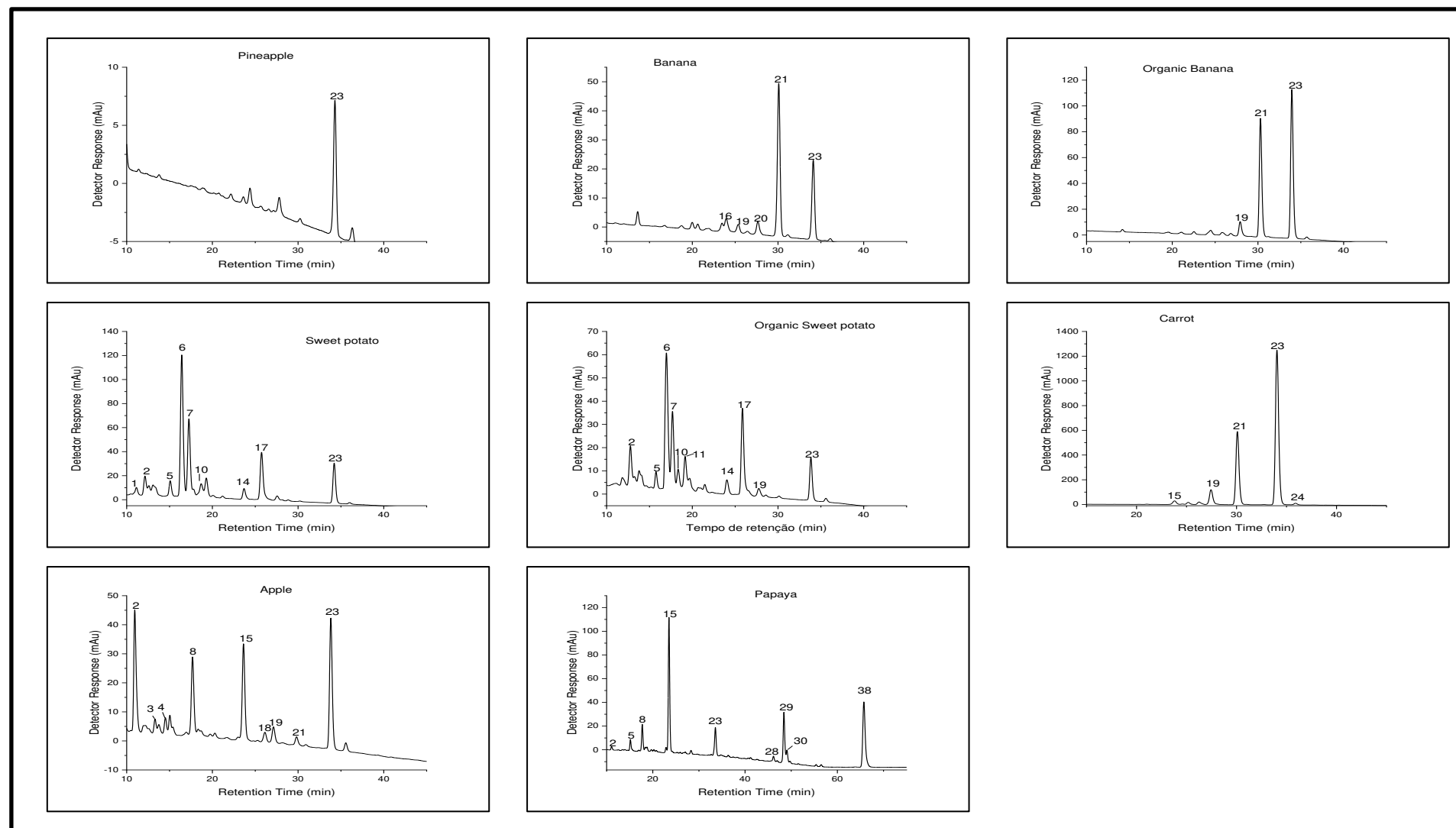
S 1. Chromatograms of fruits and vegetables before in vitro digestion, obtained from HPLC-DAD, processed at 450 nm. Peaks numbered according to Table 7
