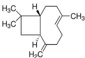
Figure 3 - Molecular structure of trans-caryophyllene.
