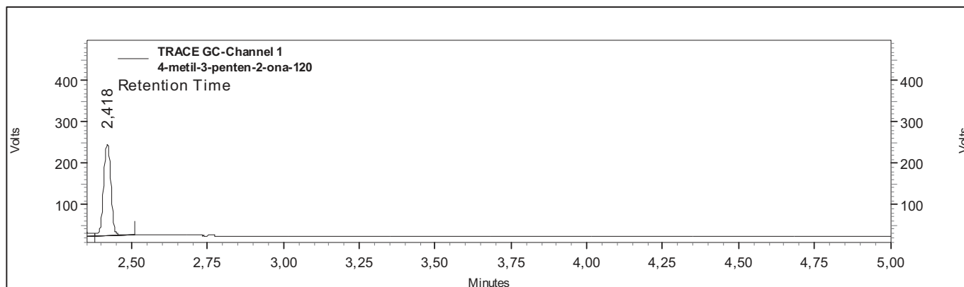
Fig. 1. GC Chromatogram of 4-Methyl-3-penten-2-one at 403.15 K.
