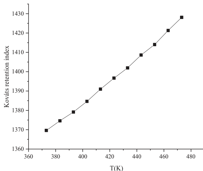
Fig. 3. Dependence of Kováts retention index on temperature for damascenone.
