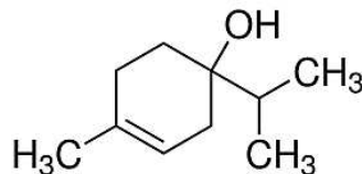
Figure 2 - Molecular structure of terpinen-4-ol.
