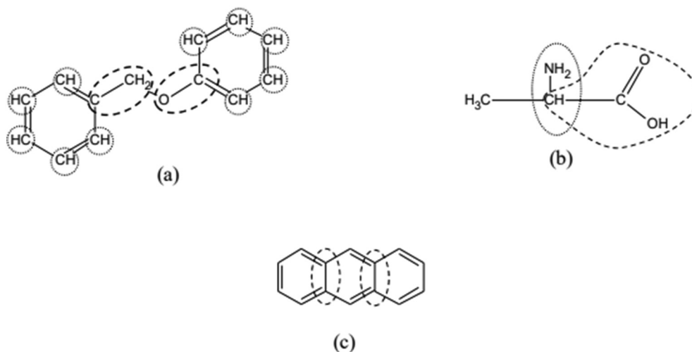
Fig. 1. Correct description of the Kolská et al. [13] method for: (a) first-order groups; (b) second-order groups; (c) third-order groups.
