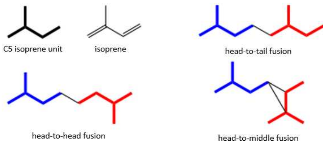
Figure 2.1 Coupling of Isoprene Units in Terpenoid Backbone Formation.
