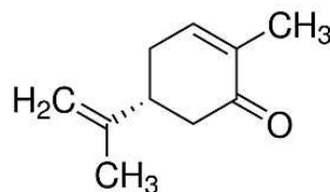
Figure 4 - Molecular structure of carvone.
