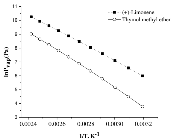
Figure 3. Temperature dependence of the vapor pressure for the monocyclic terpenes studied in this work.
