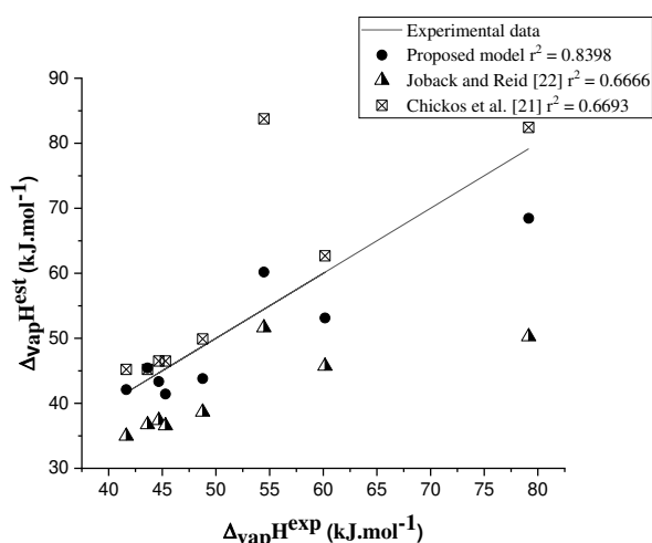
Figure 4. Enthalpies of vaporization distribution: estimated ( \Delta_{\text{vap}}H^{\text{est}} ) and experimental ( \Delta_{\text{vap}}H^{\text{exp}} ) data.
