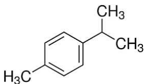
Figure 1 - Molecular structure of p-cymene.
