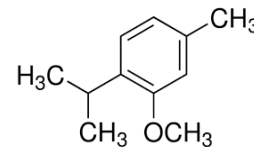
Thymol methyl ether
