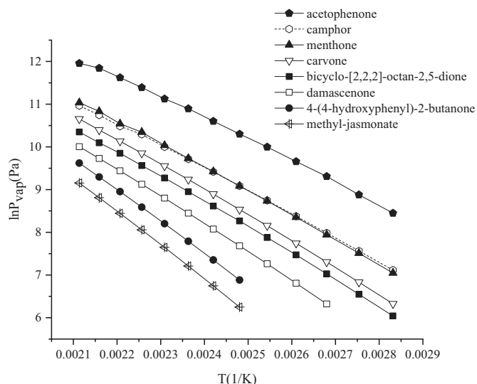
Fig. 4. Vapor pressure ( P_{vap} ) curves for aromatic and terpene ketones studied in this work.
