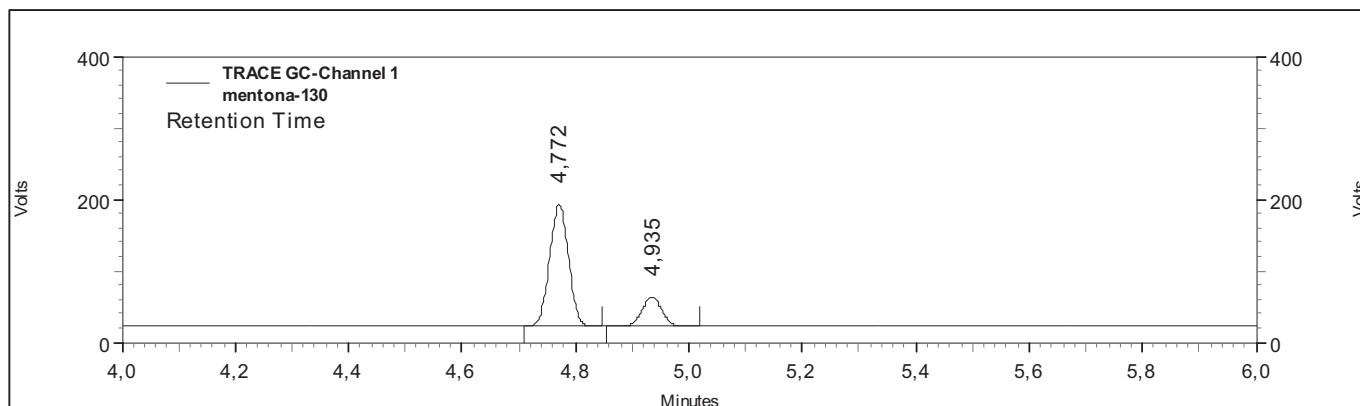
Fig. 2. GC Chromatogram of (-)-Menthone at 403.15 K (expanded from 4 to 6 minutes).
