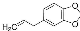
Figure 8 - Molecular structure of safrole.
