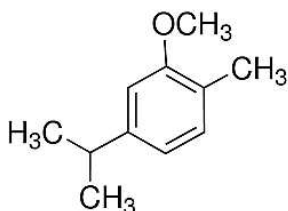
Figure 7 - Molecular structure of thymol-methyl-ether.
