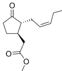
Figure 6 - Molecular structure of methyl-jasmonate.
