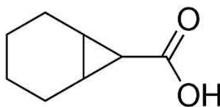
Figure 9 - Molecular structure of bicyclo[4.1.0]heptane-7-carboxylic acid.
