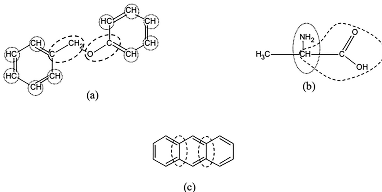
Fig. 3. Correct description of the Kolská et al. (2005) method for: (a) first-order groups; (b) second-order groups; (c) third-order groups.
