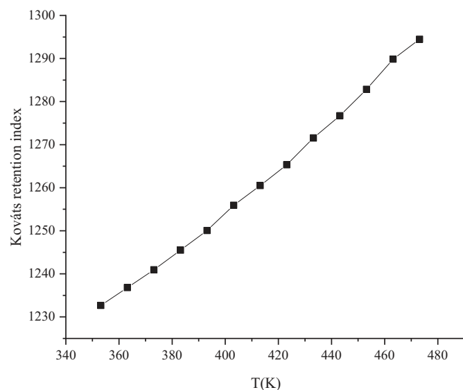
Fig. 2. Dependence of Kováts retention index on temperature for carvone.
