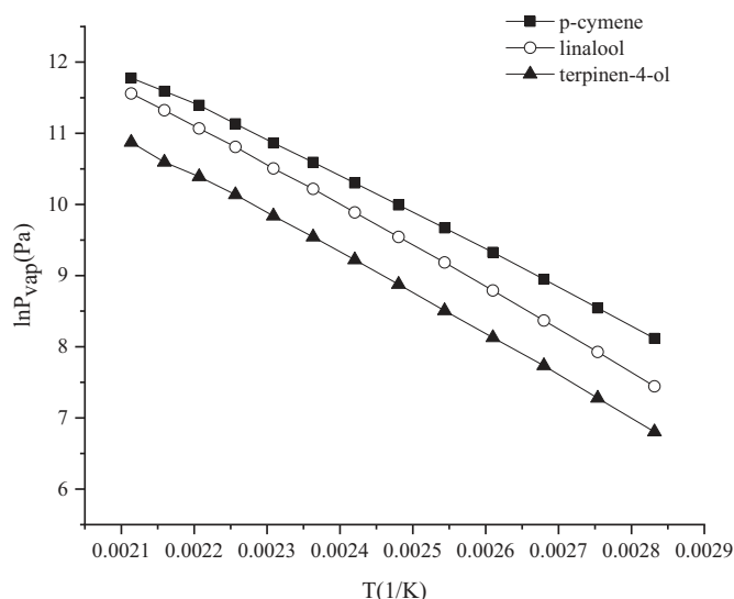
Fig. 5. Vapor pressure ( P_{vap} ) curves for hydrocarbon and other oxygenated compounds included in this study.
