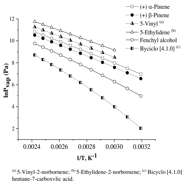
Figure 2. Temperature dependence of the vapor pressure for the bicyclic terpenes studied in this work.
