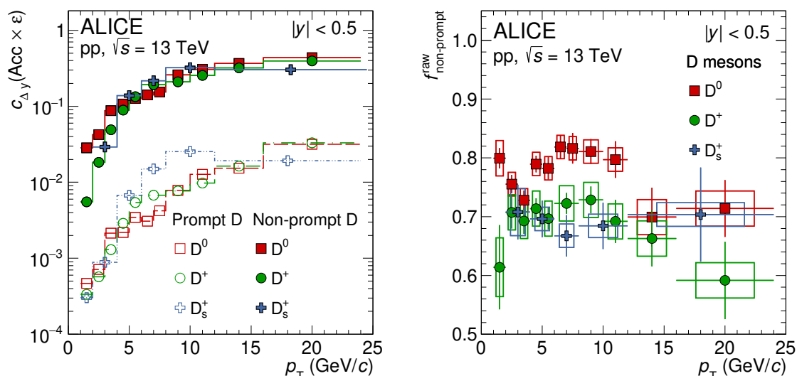
Figure 2. Left: c_{\Delta y}(\text{Acc} \times \epsilon) factors of the selection criteria of the analyses for prompt and non-prompt D mesons as a function of p_T . Right: raw fraction of non-prompt D^0 , D^+ , and D_s^+ mesons in the raw yield as a function of p_T . The vertical bars and boxes display the statistical and systematic uncertainties, respectively.
