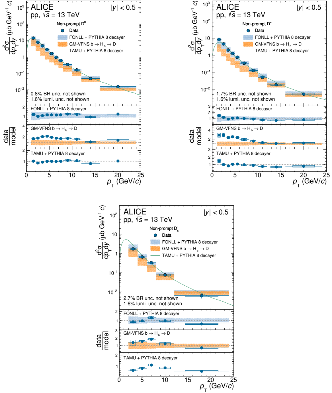
Figure 4. p_T -differential production cross sections of non-prompt D^0 (top-left), D^+ (top-right), and D_s^+ (bottom) mesons at midrapidity, |y| < 0.5 , in pp collisions at \sqrt{s} = 13 TeV compared with the predictions from FONLL + PYTHIA 8 [47, 48], GM-VFNS [41, 42], and TAMU + PYTHIA 8 [82] calculations. The lower panels report the data-to-model ratios. The vertical bars and empty boxes represent the statistical and systematic uncertainties, respectively.
