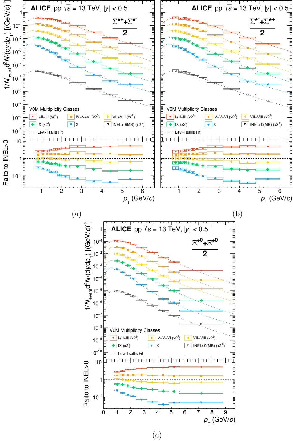
Figure 5. Transverse momentum spectra of \Sigma(1385)^+ (a), \Sigma(1385)^- (b) and \Xi(1530)^0 (c) in pp collisions at \sqrt{s} = 13 TeV in multiplicity classes and for the inclusive case ( \text{INEL} > 0 ). Statistical and total systematic uncertainties are shown by error bars and boxes, respectively. The bottom panels show the ratios of the multiplicity-dependent spectra to the \text{INEL} > 0 distributions. The systematic uncertainties on the ratios are obtained by considering only contributions of multiplicity-uncorrelated uncertainties described in table 5. The dashed lines represent the fits to the spectra with the Lévy-Tsallis function.
