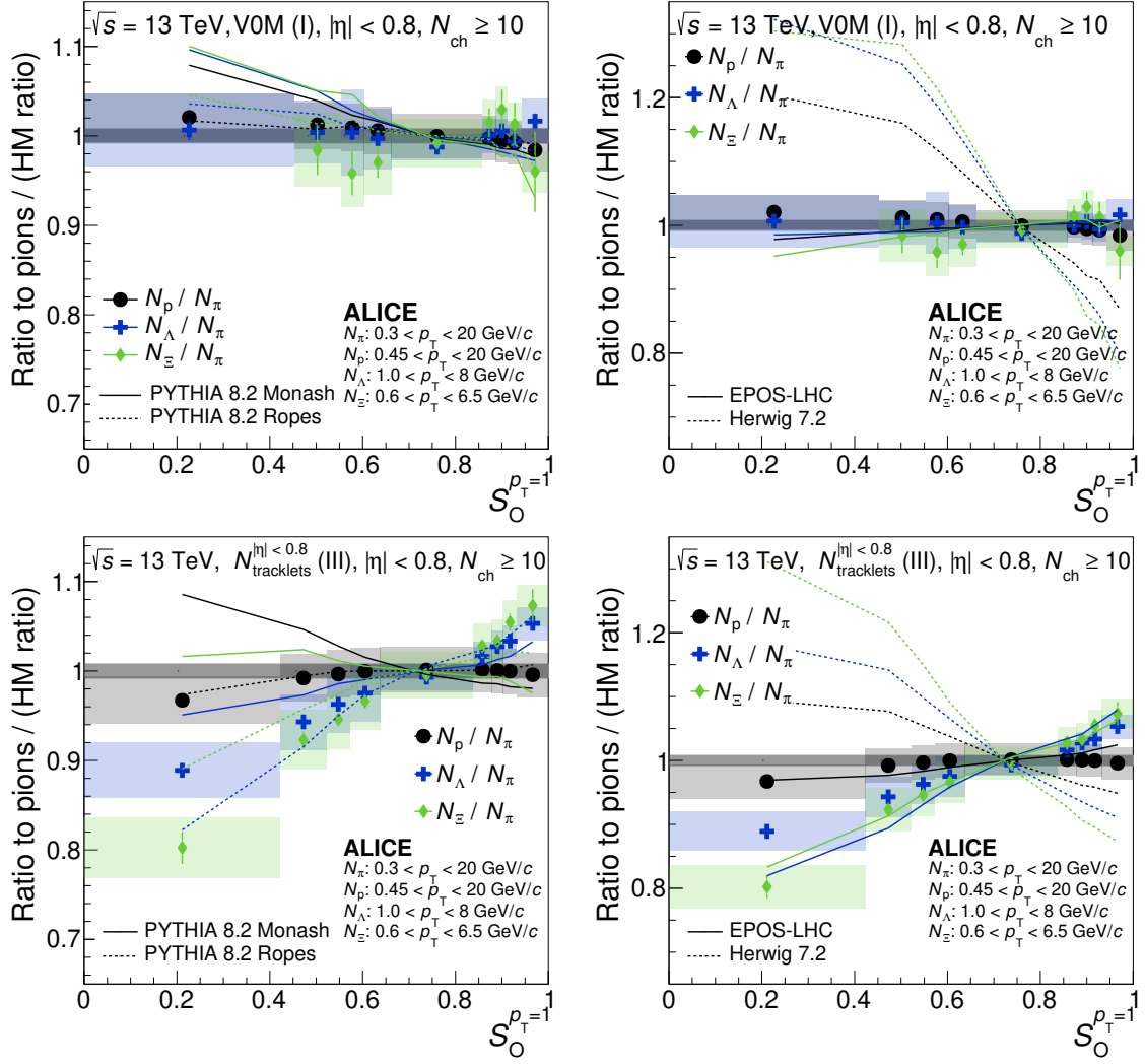
Figure 18. The double ratios of integrated yield as a function of S_O^{p_T=1} are presented for V0M 0–1% (upper) and N_{\text{tracklets}}^{|\eta| < 0.8} 0–10% (lower). Left and right panels show the same data points, but with different model predictions. Statistical and total systematic uncertainties are shown by bars and boxes, respectively. The curves represent different model predictions of the same measurement.
