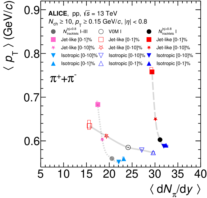
Figure 2. Correlation between \langle p_T \rangle and \langle dN_\pi/dy \rangle as a function of S_O^{p_T=1} , in the 0–10% and 0–1% V0M and N_{tracklets}^{|\eta| < 0.8} multiplicity classes. The total systematic uncertainties are represented by empty boxes. The statistical uncertainty is smaller than the reported marker sizes.
