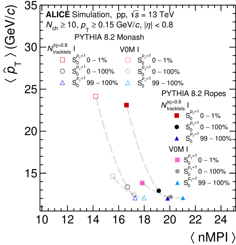
Figure 3. PYTHIA 8.2 correlation study between \langle \hat{p}_T \rangle and \langle n_{MPI} \rangle as a function of S_0^{p_T=1} , in 0–1% V0M and N_{tracklets}^{|\eta| < 0.8} multiplicity classes. The default PYTHIA 8.2 Monash variation is compared to PYTHIA 8.2 with color rope hadronization. The total systematic and statistical uncertainties are smaller than the marker sizes. The grey band is an interpolation between the points, to more clearly illustrate the trend of each multiplicity and model variation.
