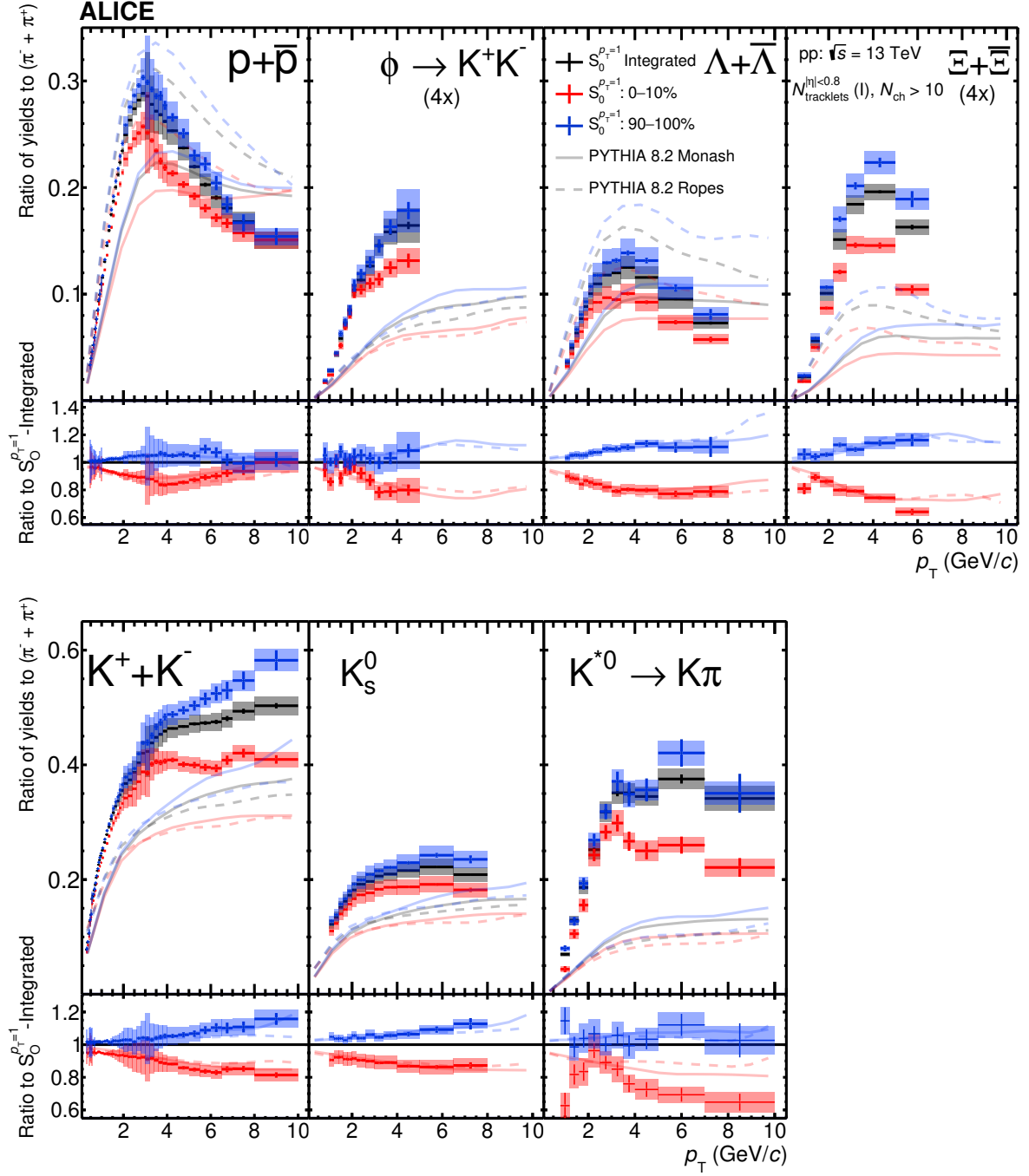
Figure 7. Top panels show hadron-to- \pi ratios for 0–10% S_O^{p_T=1} classes selected for the 0–1% N^{\text{tracklets}}_{|\eta| < 0.8} multiplicity events. Bottom panels present the hadron-to- \pi double ratios of S_O^{p_T=1} classes relative to S_O^{p_T=1} integrated high-multiplicity events. Statistical and systematic uncertainties are shown by bars and boxes, respectively. Experimental results are compared with predictions from PYTHIA 8.2 Monash and Ropes.
