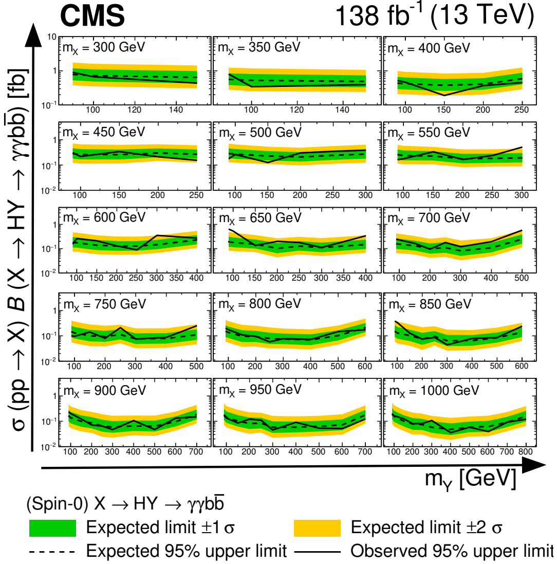
Figure 7. Expected and observed 95% CL exclusion limit on production cross section for \text{pp} \rightarrow X \rightarrow \text{HY} \rightarrow \gamma\gamma b\bar{b} signal. The dashed and solid black lines represent expected and observed limits, respectively. The green and yellow bands represent the \pm 1 and \pm 2 standard deviations for the expected limit. The middle plot in the 3rd row shows the largest excess observed for m_X = 650 \text{ GeV} and m_Y = 90 \text{ GeV} .
