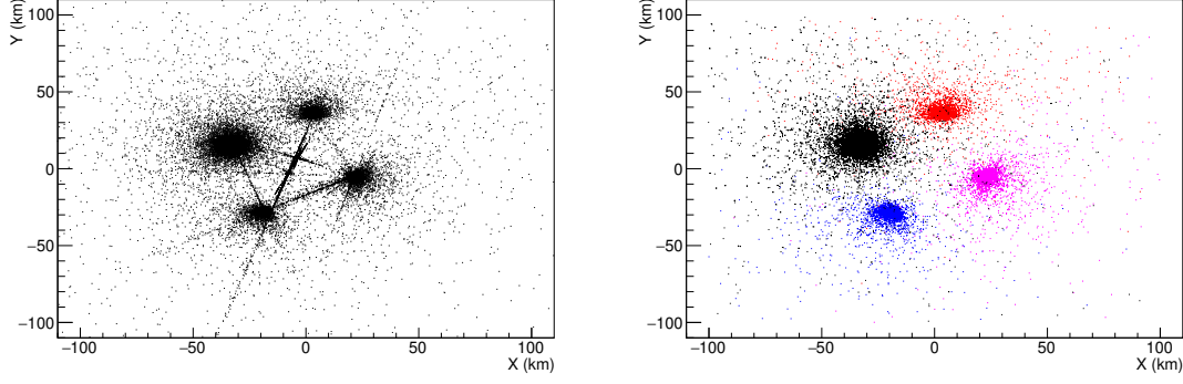
Figure 3: Distribution of the exit point of the events in the burn sample before (left) and after (right) the laser identification and rejection. The straight lines, related to laser events, are correctly removed and only clusters of events remained close to each of the FD sites.
