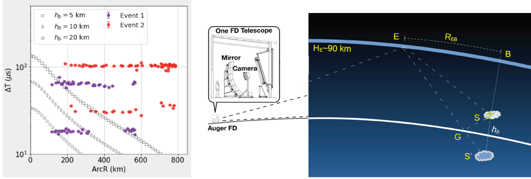
Figure 5: Left: time gaps between flashes in two typical triple ELVES events vs arcdistance R_{EB} from the vertical of the source and the point of light emission; Right: geometrical model for the calculation of the time gap.
