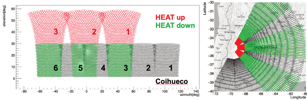
Figure 6: Field of view of the HEAT telescopes in operation mode (red) and in calibration mode (green), compared to the Coihueco telescopes.
