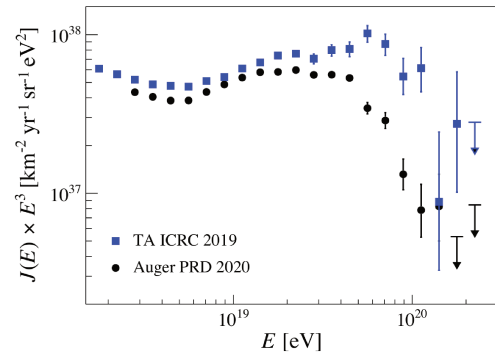
Figure 1: Measured UHECR flux: Auger (black circles) and TA (blue squares) (adapted from [3]).
