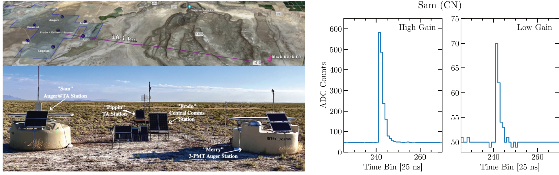
(a) Top: Location of the 9 station micro-array within TA, also showing the distance to the Black Rock FD. Bottom: Center triplet and data acquisition comms station. Station names inspired by [18]. (b) High gain (left) and low gain (right) channel signal traces obtained from the WCD PMT of the Auger@TA central triplet station.
