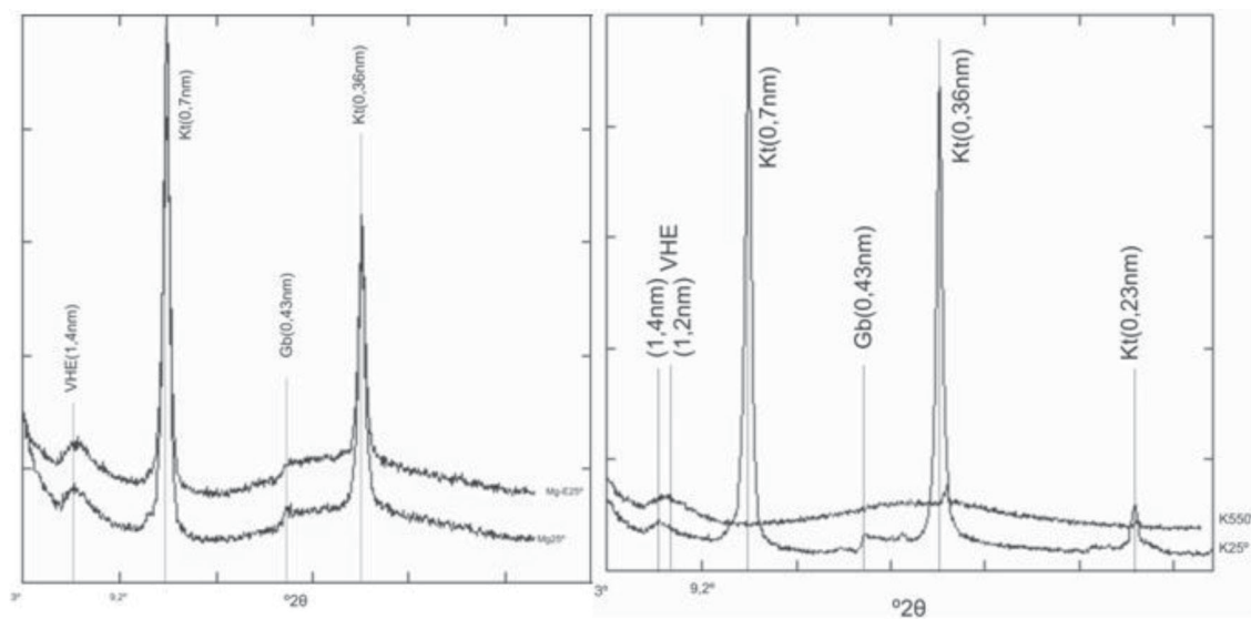
FIGURE 12. Clay Fraction from the oriented thin section method. Left: MgCl_2 -saturated solution at 25°C and solvated with E-Glycol. Right: KCl-saturated solution at 25°C and 550°C. The values in parenthesis are the d-spacings in nm. Kt: Kaolinite; Gb: Gibbsite; VHE: Hidroxy-Interlayered Vermiculite.
