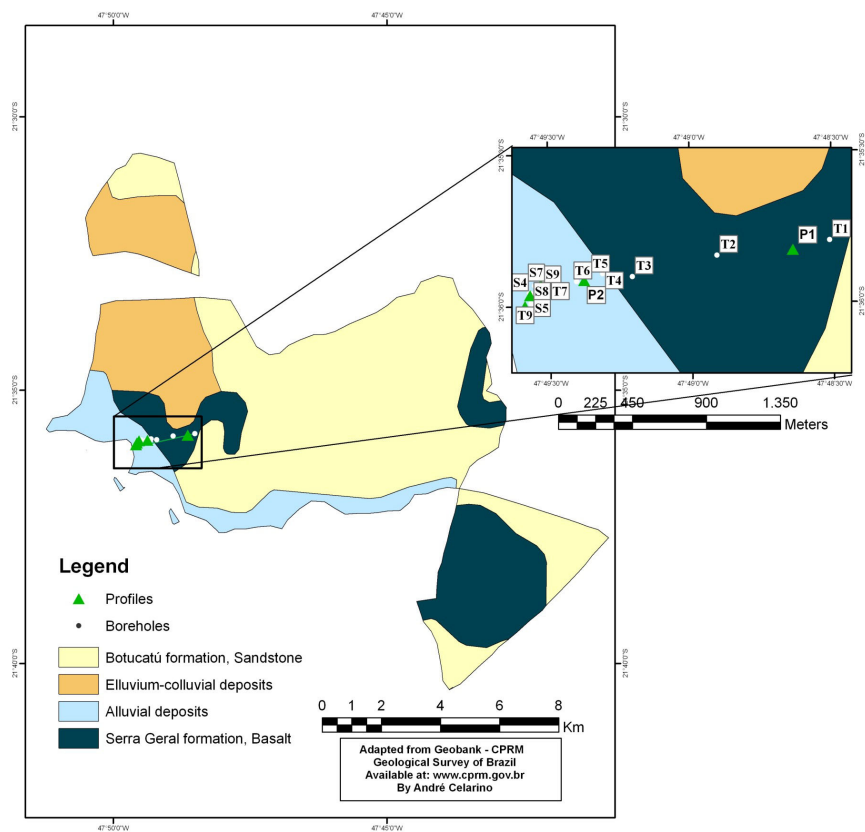
FIGURE 4. Geologic map of the study area.
