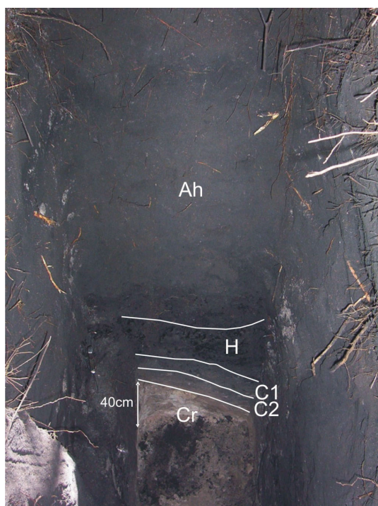
FIGURE 13. Typic Udifluvent (LDEH) profile.
