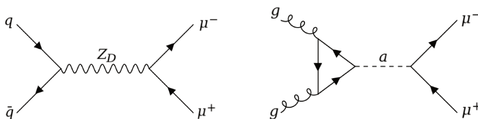
Figure 1. Expected dominant production modes for beyond-SM particles: a dark photon Z_D (left) and light pseudoscalar boson a (right).
