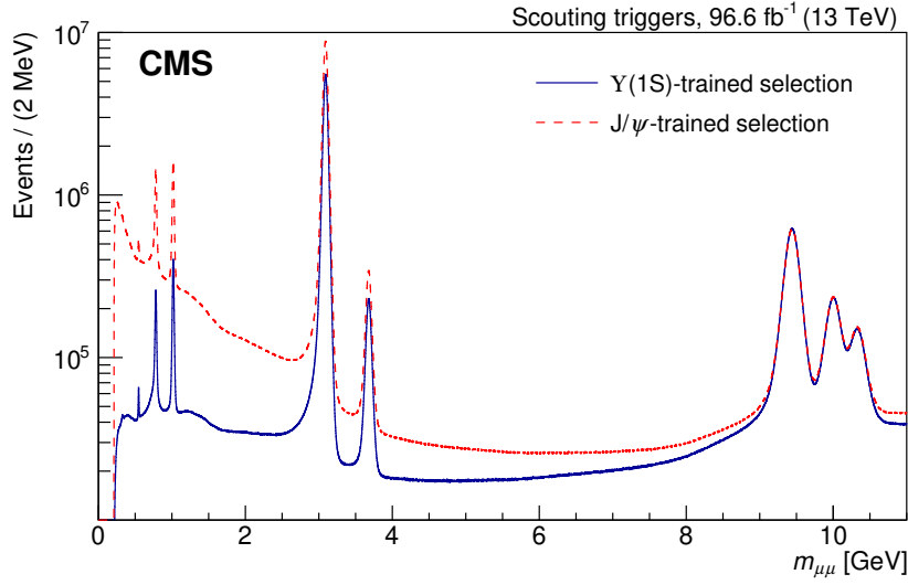
Figure 3. The m_{\mu\mu} distribution obtained with the muon scouting data collected during 2017–2018 with two sets of selections: the Y(1S)-trained muon MVA identification with L_{xy} < 0.015 cm (blue, solid), and the J/ψ-trained muon MVA identification with L_{xy}/\sigma_{L_{xy}} < 3.5 (red, dashed). The J/ψ-trained and Y(1S)-trained selections are used in the mass range 1.1–2.6 and 4.2–7.9 GeV, respectively.
