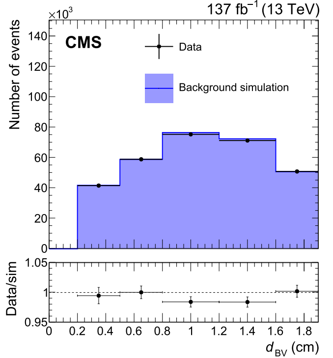
FIG. 5. The distribution of d_{\text{BV}} in K_S^0 vertices in data (black) and simulation (purple). The lower panel shows the ratio between data and simulation.
