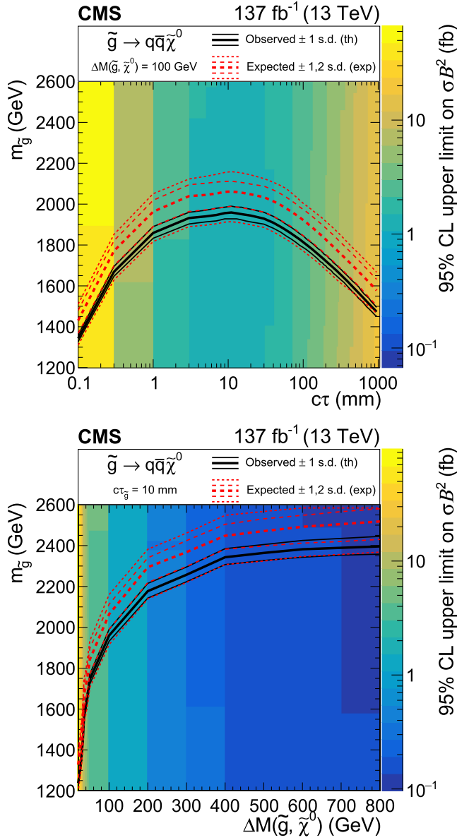
FIG. 8. Upper: the 95% \text{CL}_s upper limit on the product of the cross section and branching fraction squared for the split-SUSY signal model with a mass splitting of 100 GeV, shown as a function of gluino mass and c\tau . Lower: the 95% \text{CL}_s upper limit on the product of the cross section and branching fraction squared for the split-SUSY model with a c\tau of 10 mm, shown as a function of gluino mass and mass splitting. For both plots, the observed (solid black) and expected (dashed red) exclusion curves are shown.
