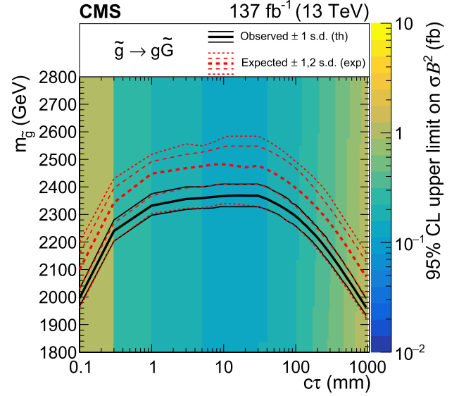
FIG. 9. The 95% \text{CL}_s upper limit on the product of the cross section and branching fraction squared for the GMSB SUSY signal model, shown as a function of gluino mass and c\tau . The observed (solid black) and expected (dashed red) exclusion curves are shown.
