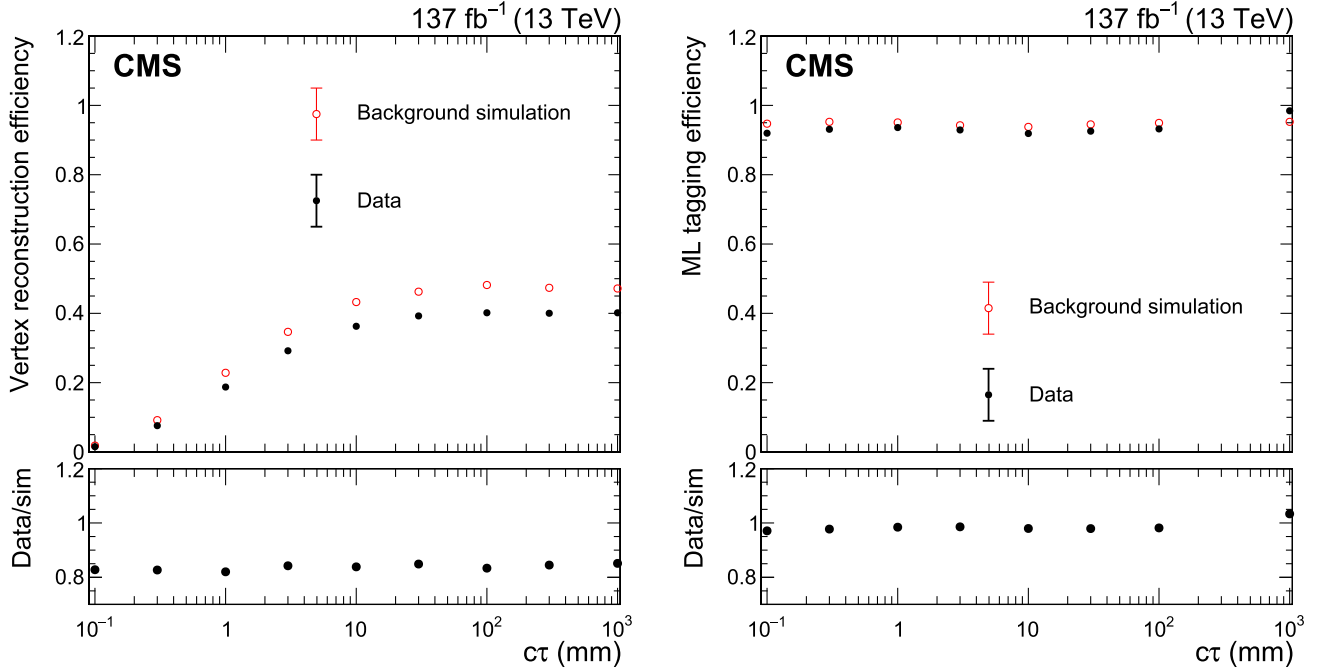
FIG. 6. The vertex reconstruction efficiency (left) and ML tagging efficiency (right) for artificially displaced vertices in data (black) and simulation (red). In this example, the artificially displaced vertices are corrected to mimic split-SUSY signal events with gluino mass of 2000 GeV and neutralino mass of 1800 GeV. The uncertainties are too small to be visible in the plot.
