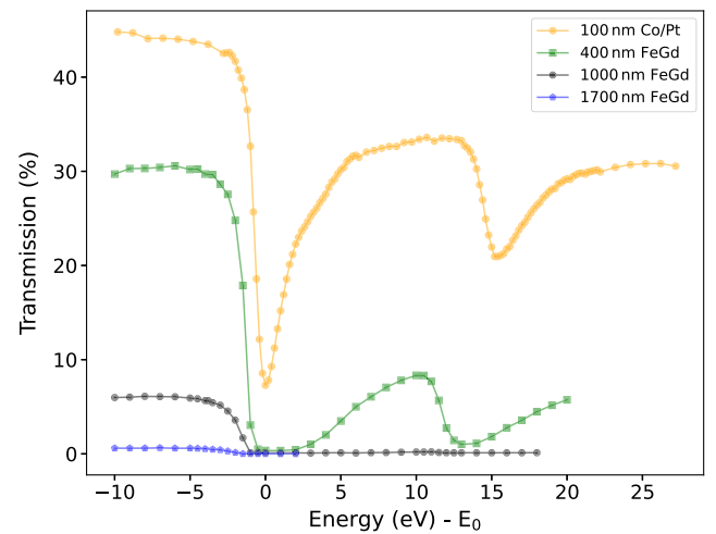
FIG. 11. Transmission signal through the thickness of the 100-nm-thick CoPt multilayer (yellow), 400 nm (green), 1 \mu\text{m} (black), and 1.7 \mu\text{m} (blue) FeGd samples. The energies are normalized with respect to the L_3 absorption edge of the materials at 780 eV for Co and 710 eV for Fe. Nonzero transmission is measurable only at preabsorption edges for the thick FeGd samples. On-resonance, the transmission is zero.
