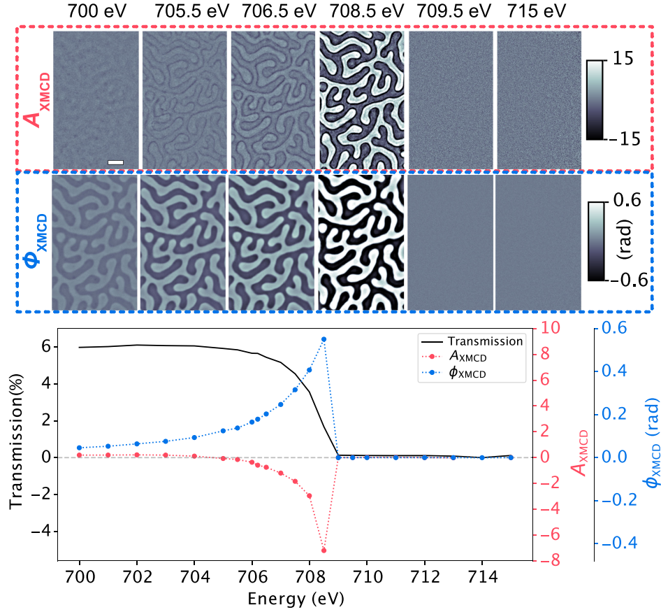
FIG. 12. Pre-edge phase ptychography on 1- \mu m-thick FeGd samples close to the Fe L_3 edge. Complex XMCD spectrum across the Fe L_3 edge extracted from magnetic domains in XMCD projections of a 1- \mu m-thick FeGd film with A_{\text{XMCD}} and \phi_{\text{XMCD}} shown as red and blue dots, respectively. The black line indicates the transmission through the sample. The images above the plot show A_{\text{XMCD}} and \phi_{\text{XMCD}} images for a few selections of energies. The scale bar represents 500 nm.
