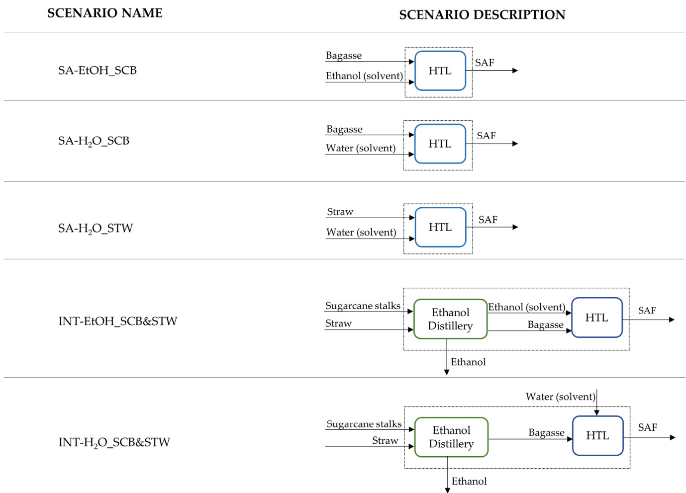
Figure 1. Simplified fluxograms of the proposed scenarios. Solvent varies according to each scenario: for SA-EtOH_SCB, the solvent is anhydrous ethanol (purchased from surrounding mills) and for the INT-EtOH_SCB&STW scenario, ethanol is diverted from the distillery that is integrated into HTL plant. For the SA-H 2 O_SCB, SA-H 2 O_STW, and INT- H 2 O_SCB&STW scenarios, the solvent is water.
