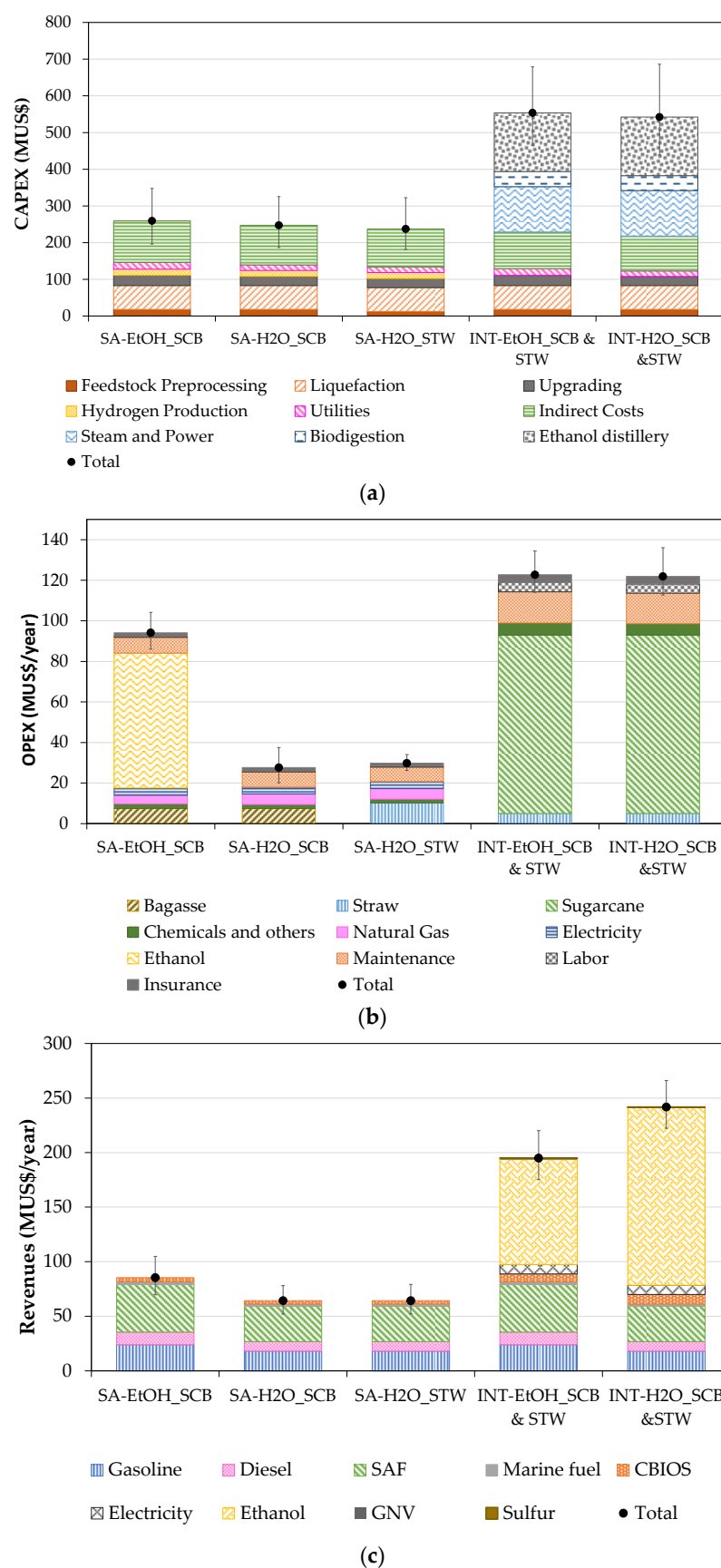
Figure 2. Economic results: (a) CAPEX (MUSD), (b) OPEX (MUSD/year), and (c) revenues (MUSD/year).
