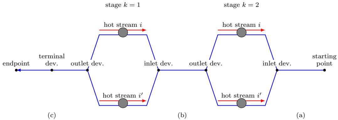
Figure 4.15: The topology of cold stream j running from left to right in a two-stage superstructure.
