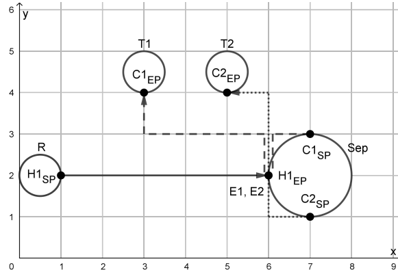
Figure 3.8: The heat exchangers overlapping each other and also an endpoint.
