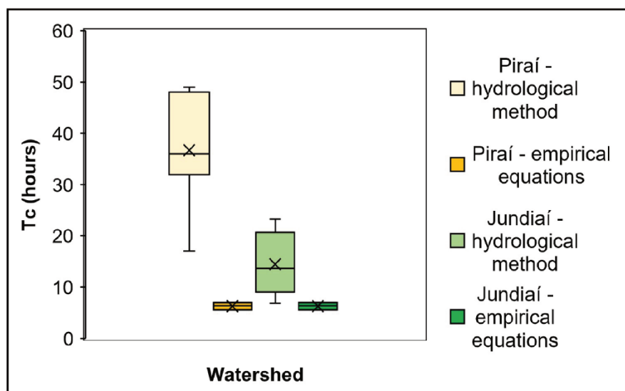
Figure 6 – Comparison between the time of concentration calculated from hydrological data and by empirical equations, for Pirai and Jundiaí watersheds
