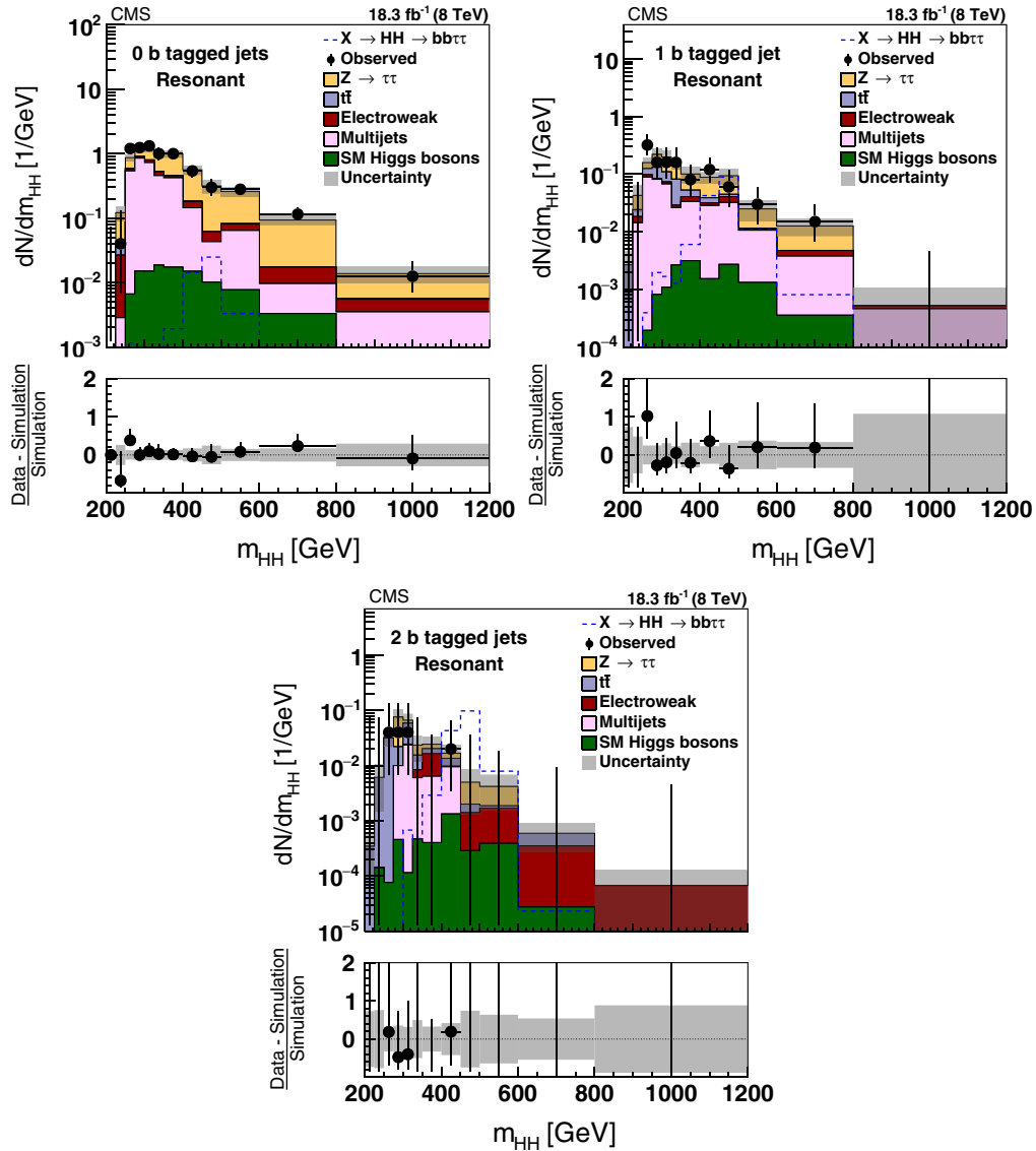
FIG. 4. Distributions in m_{HH} observed in the event categories with 0 b tags, 1 b tag, and 2 b tags in the data compared to the background expectation. Hypothetical signal distributions corresponding to the decays of a spin 2 resonance X of mass m_X = 500 GeV that is produced with a \sigma(pp \rightarrow X)\mathcal{B}(X \rightarrow HH) of 1 pb are overlaid for comparison. The corresponding WED model parameters are kl = 35 and k/\bar{M}_{Pl} = 0.2 . The expectation for signal and background processes is shown for values of nuisance parameters obtained from the likelihood fit.
