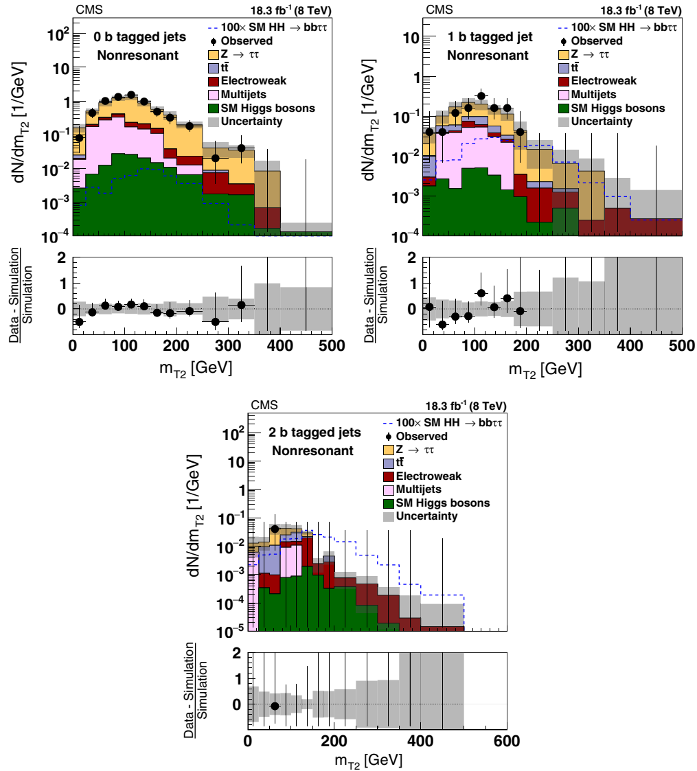
FIG. 3. Distributions in m_{T2} observed in the event categories with 0 b tags, 1 b tag, and 2 b tags in the data compared to the background expectation. Hypothetical nonresonant HH signals with a cross section \sigma(pp \rightarrow HH) of 1 pb, corresponding to 100 times the SM cross section are overlaid for comparison. The expectation for signal and background processes is shown for values of nuisance parameters obtained from the likelihood fit.
