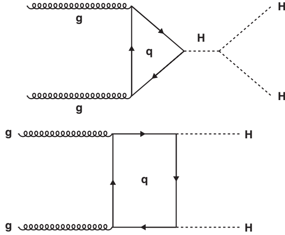
FIG. 1. LO Feynman diagrams for HH production within the SM.
