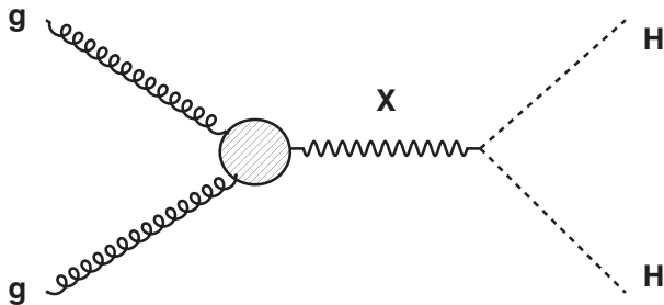
FIG. 2. LO process for the production of a pair of H 's through the decay of a heavy resonance X .
