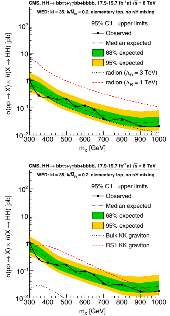
FIG. 6. 95% CL observed and expected upper limits on the cross section times branching fraction [ \sigma(pp \rightarrow X)\mathcal{B}(X \rightarrow HH) ] for a spin 0 (upper) and for a spin 2 (lower) resonance X as functions of the resonance mass m_X , obtained from the combination of searches performed in the bb\tau\tau , \gamma\gamma bb and bbbb decay channels. The green and yellow bands represent, respectively, the 1 and 2 standard deviation extensions beyond the expected limit. Also shown are theoretical predictions corresponding to WED models for radions for values of \Lambda_R = 1, 3 and for RS1 and Bulk KK gravitons [18,19]. The other WED model parameters are kl = 35 and k/\bar{M}_{\text{Pl}} = 0.2 , assuming an elementary top hypothesis and no radion-Higgs ( r/H ) mixing.
