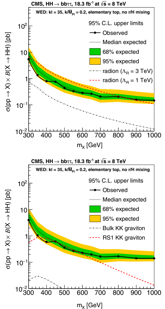
FIG. 5. The 95% CL observed and expected upper limits on the \sigma(pp \rightarrow X)\mathcal{B}(X \rightarrow HH) for a spin 0 (upper) and for a spin 2 (lower) resonance X as functions of the resonance mass m_X , obtained from the search in the decay channel bb\tau\tau . The green and yellow bands represent, respectively, the 1 and 2 standard deviation extensions beyond the expected limit. Also shown are theoretical predictions corresponding to WED models for radions for values of \Lambda_R = 1, 3 TeV and for RS1 and bulk KK gravitons [18,19]. The other WED model parameters are kl = 35 and k/\bar{M}_{\text{Pl}} = 0.2 , assuming an elementary top hypothesis and no radion-Higgs ( r/H ) mixing.
