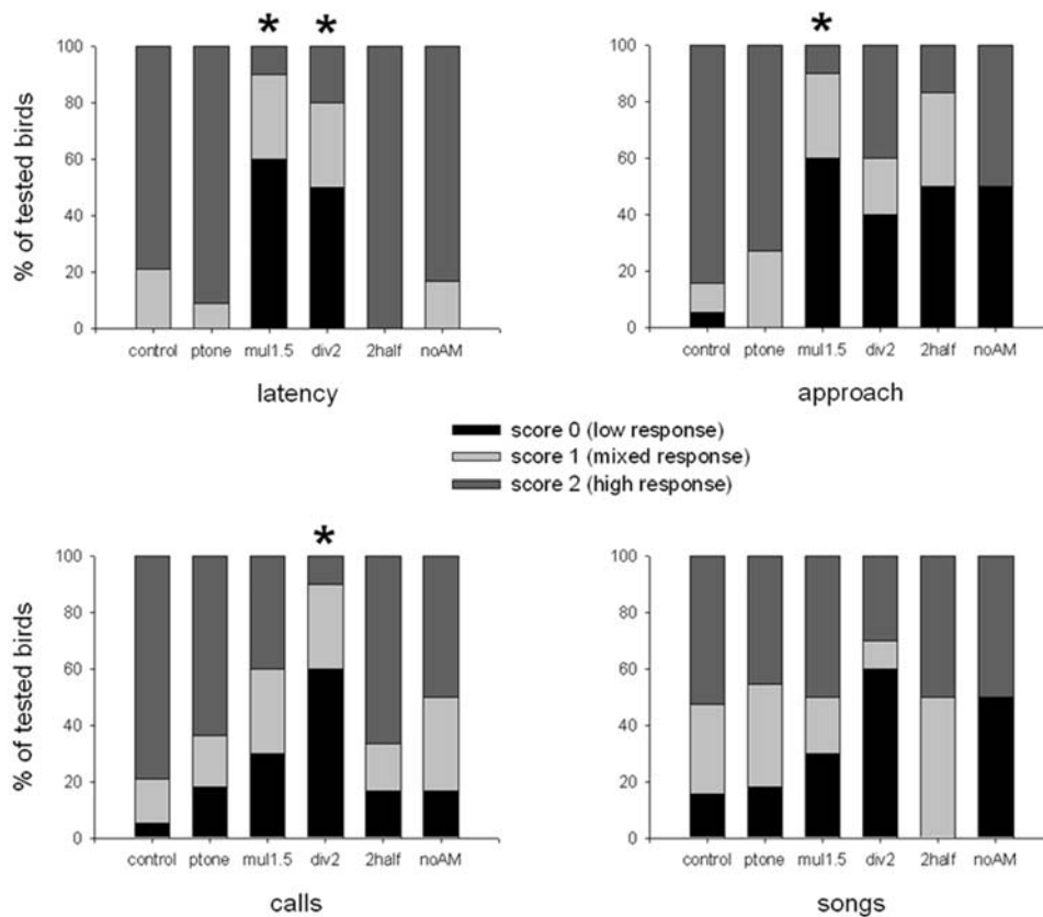
Figure 2. Behavioral responses to experimental signals. (control=control song, n=19 birds; ptone=synthetic continuous pure tone, n=11 ; mul1.5=slope multiplied by 1.5, n=10 ; div2=slope divided by 2, n=10 ; 2half=second half of the song, n=6 ; noAM=without AM song, n=6 ). Results of Kruskal-Wallis tests: latency, H(5, n=62)=34.38, P=0.000 ; approach, H(5, n=62)=22.24, P=0.000 ; calls, H(5, n=62)=15.94, P=0.007 ; songs, H(5, n=62)=4.55, P=0.473 . *: significant difference with control (post-hoc multiple comparison tests; see text for details). doi:10.1371/journal.pone.0001580.g002
