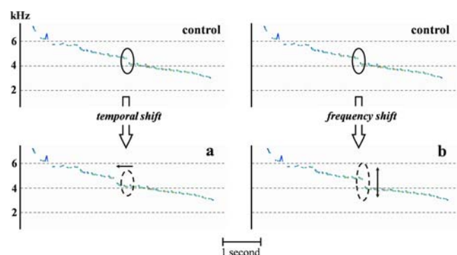
Figure 4. Experimental songs with the position of the main frequency "gap" modified. a, in the time domain. b, in the frequency domain. doi:10.1371/journal.pone.0001580.g004
