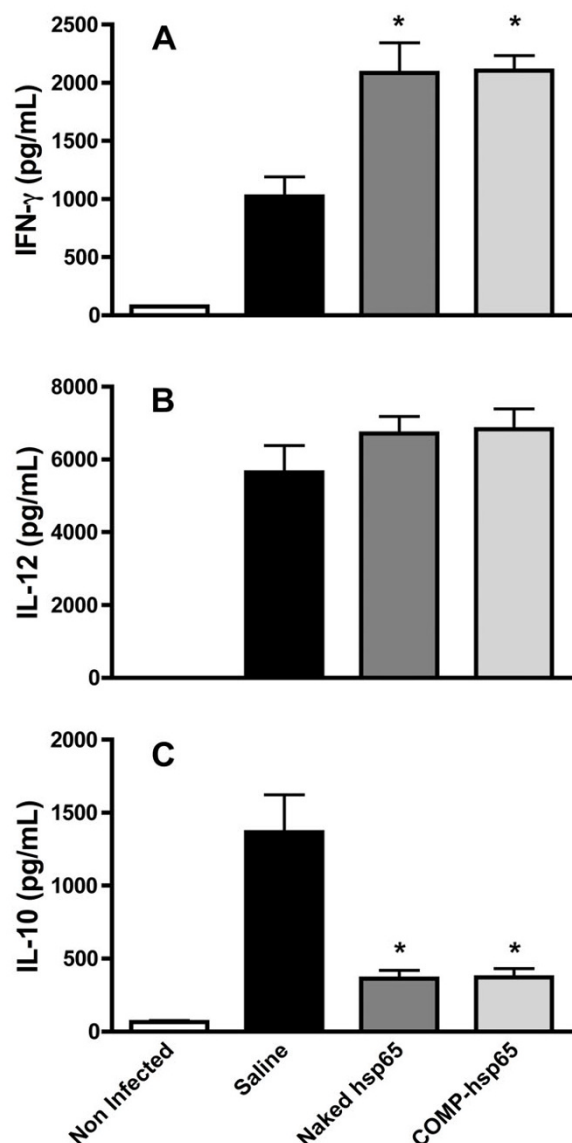
Figure 7 Cytokine production from the lung tissue of mice immunized with naked DNA-hsp65 or carried by liposome. Mice were immunized by intramuscular injection with naked hsp65 (400 µg) or by intranasal instillation with COMP-hsp65 (one dose of 25 µg). Thirty days after the last dose, mice were challenged intra-tracheally with M. tuberculosis H37RV and 30 days post infection, IFN-γ (A), IL-12 (B) and IL-10 (C) levels were determined by ELISA in lung homogenate. Data represent the mean ± SD of six mice per group of one of three independent experiments. *p < 0.01 were considered significant when compared to the saline group.
