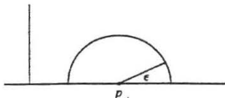
Semi-disco \bar{D}(p, \varepsilon)
