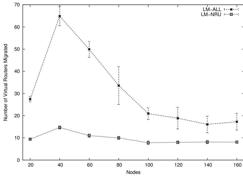
Figure 5.7: Average Virtual Routers Migrated per Event of Virtual Network Termination
