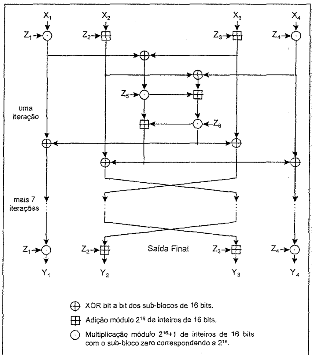
Figura 4.8 - IDEA [Schneier 96].
