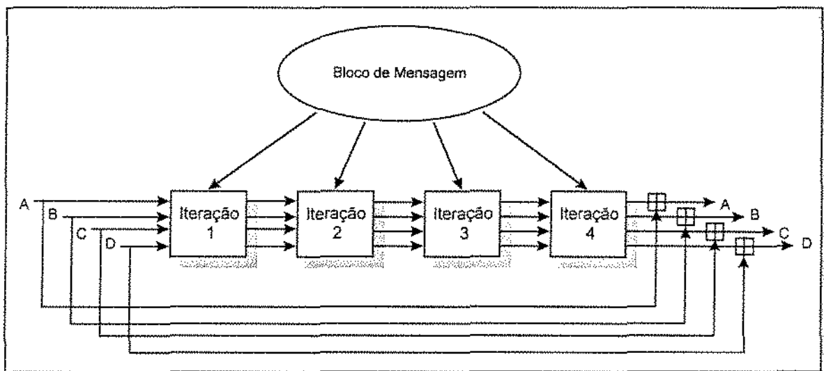
Figura 4.10 - Loop Principal do MD5 [Schneier 96].
