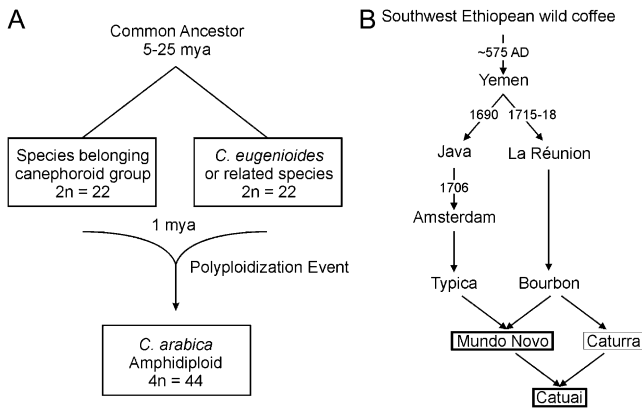
Figure 1. Evolutionary history of allotetraploid C. arabica . A, Origin of C. arabica . The progenitor genomes are represented by diploid C. eugenioides and C. canephora . C. arabica arose 1 to 2 million years ago (mya) from the fusion of C. canephora (or related species) and C. eugenioides . B, Origin of cultivated cultivars of C. arabica (based on Anthony et al., 2002).
