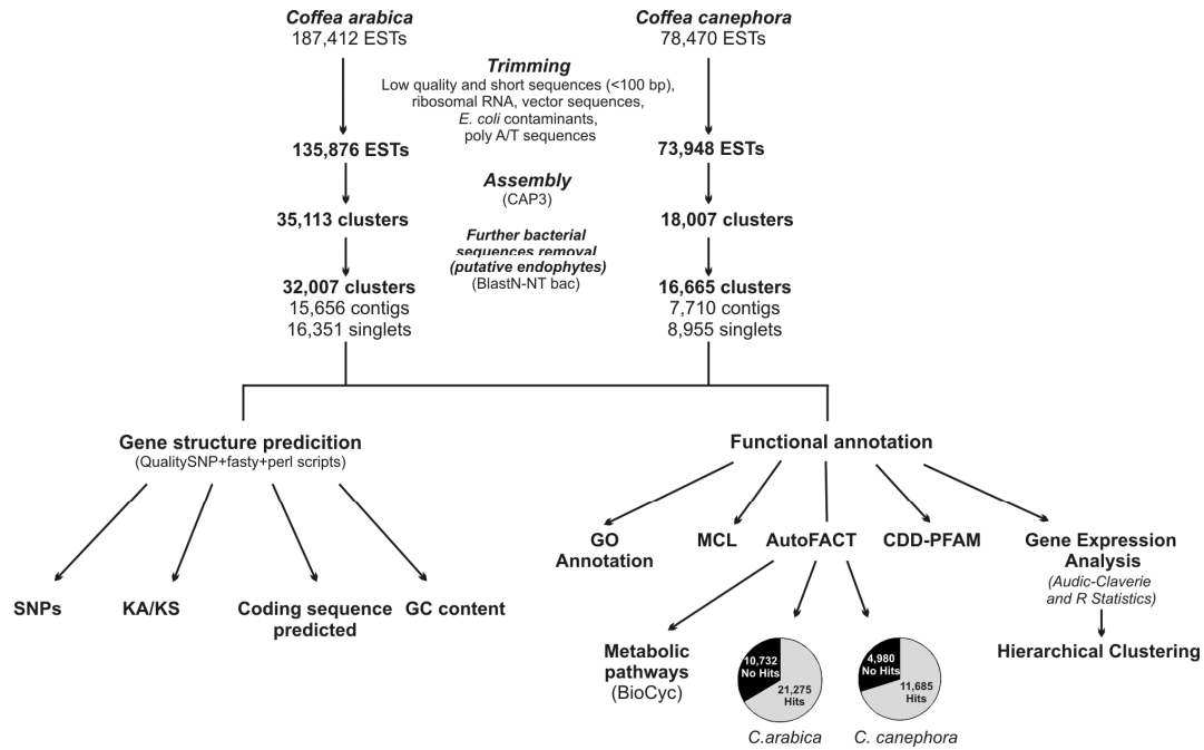
Figure 1. Flow diagram of bioinformatics procedures applied in C. arabica and C. canephora transcriptomic analyses.
