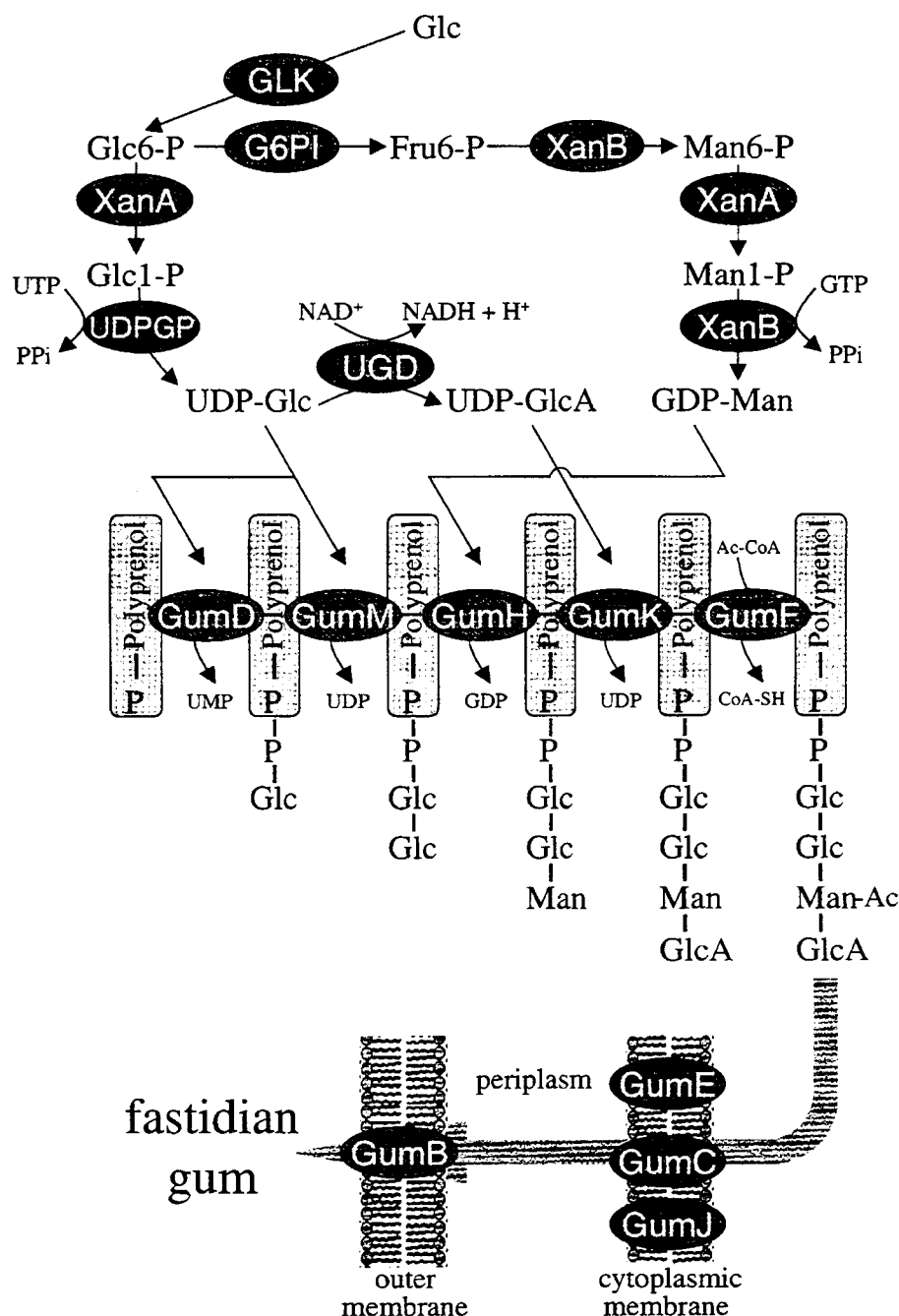
Fig. 2. Proposed synthesis pathway for fastidians gum. Putative proteins are shown in the gray ovals. The names of the enzymes correspond to those shown in Table 1. The arrows for the sequential reactions which add sugars to polyphenol are not shown. Glc, D-glucose; GlcA, D-glucuronic acid; Man, D-mannose; Ac, acetyl ester; PPi, pyrophosphate.
