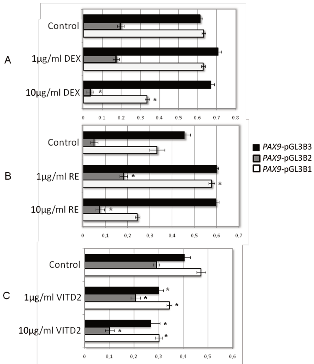
Figure 4. Functional analysis of PAX9 gene promoter by the Dual luciferase assay in MCF-7 cells. Luciferase activity in MCF-7 cells transfected with PAX9-pGL3B1 , PAX9-pGL3B2 , PAX9-pGL3B3 and pRL-TK as a control under Dexamethasone (DEX) (4A), Retinoic Acid (RE) (4B) and Ergocalciferol (VITD2) (4C) treatment.
