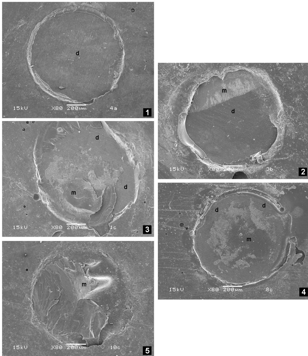
Figure 3 - Representative samples of each failure pattern in accordance with used scores (original magnification: \times 80 ), “m” representing the remaining material and “d” the area where dentine was exposed.
