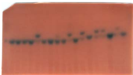
Leucina amino peptidase (LAP)
