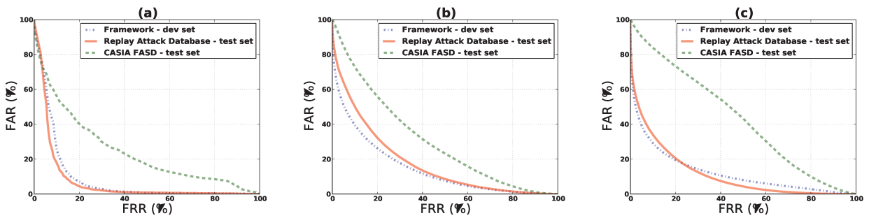
Figure 4.8: ROC curves of each countermeasure trained with the Score Level Fusion based Framework (a) Correlation with frame differences (b) LBP - TOP countermeasure (c) LBP countermeasure.
