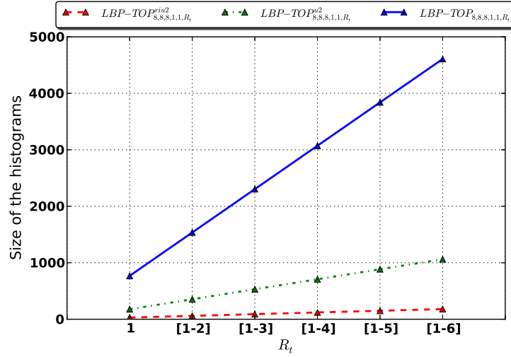
Figure 3.10: Evaluation of the histogram size when ( R_t ) is increased.
