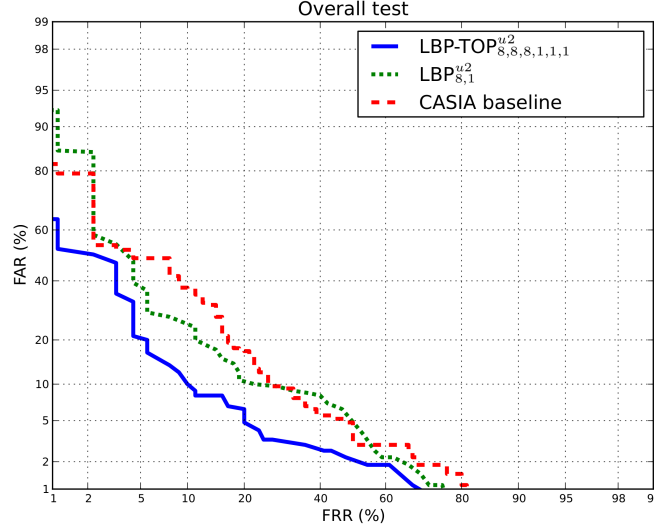
Figure 3.13: Overall performance of \text{LBP-TOP}_{8,8,8,1,1,1}^{u2} using average of features compared to the DoG baseline method and \text{LBP}_{8,1}^{u2} on the CASIA FASD.
