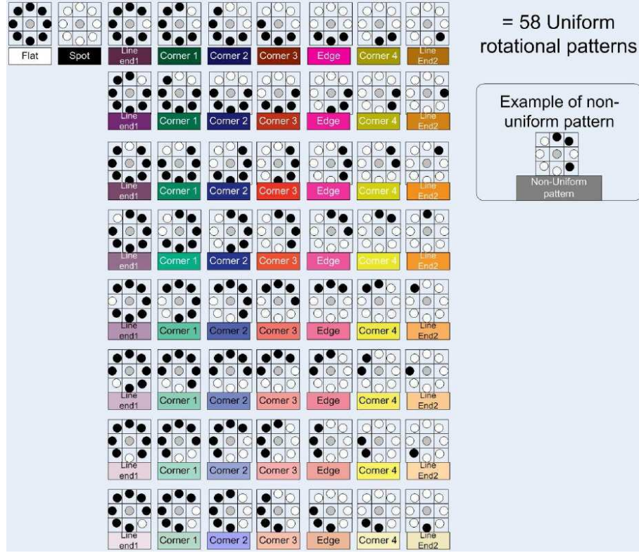
Figure 3.2: All uniform patterns for LBP with 8 neighbours Chan et al. (2007).
