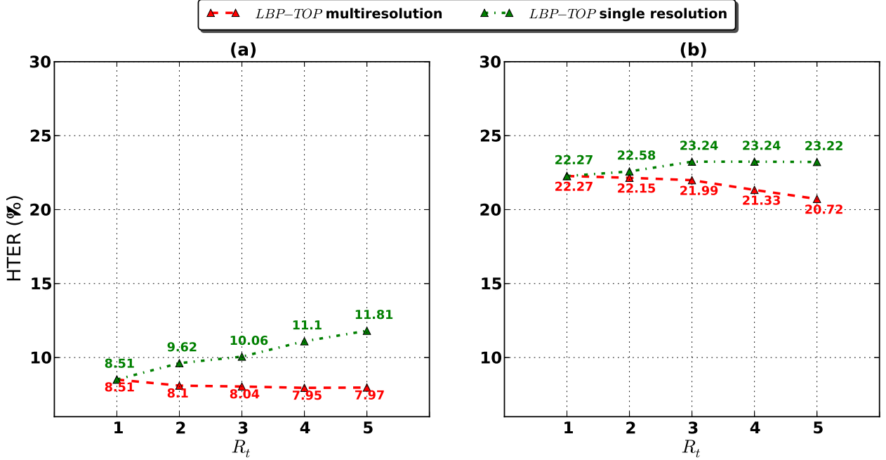
Figure 3.11: HTER(%) evaluation using LBP-TOP u2 8,8,8,1,1, R_t with the single resolution and the multiresolution approach using SVM classifier (a) Replay Attack Database (b) CASIA FASD.
