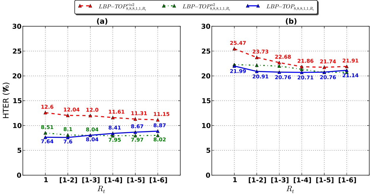
Figure 3.9: HTER(%) evaluation with LBP-TOP_{8,8,8,1,1,R_t} using different LBP operators in the planes with SVM classifier (a) Replay Attack Database (b) CASIA FASD.
