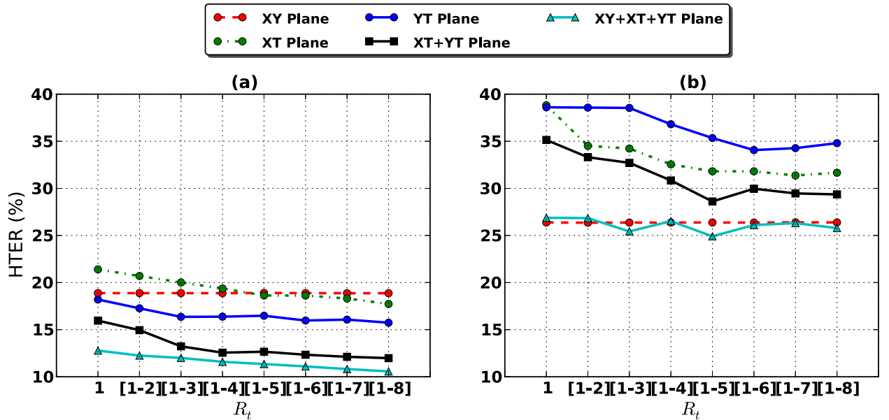
Figure 3.7: HTER(\%) evaluation in each plane when the multiresolution area ( R_t ) is increased with LBP-TOP_{8,8,1,1,R_t}^{u2} and LDA classifier - test-set (a) Replay Attack Database (b) CASIA FASD.
