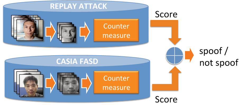
Figure 4.7: Score Level Fusion based Framework schema
