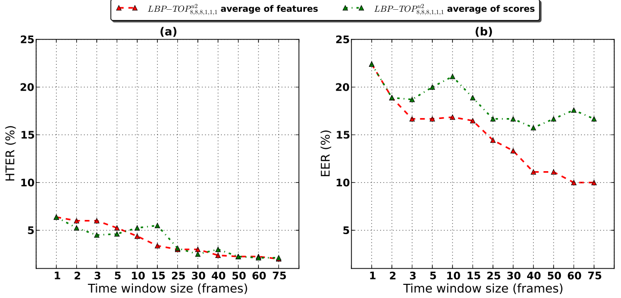
Figure 3.12: Access attempt based evaluation of different time window sizes using mean of features and mean of scores with LBP-TOP 8,8,1,1,1 u2 (a) Replay Attack Database (HTER %) (b) CASIA FASD (EER %).
