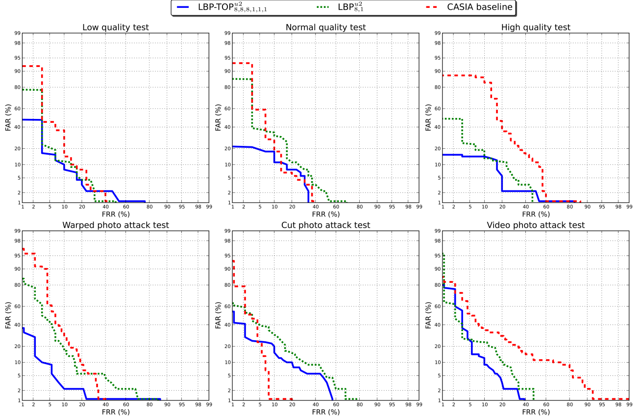
Figure 3.14: Performance of LBP-TOP_{8,8,1,1,1}^{u2} using average of features compared to the DoG baseline method and LBP_{8,1}^{u2} under the different protocols of the CASIA FASD.
