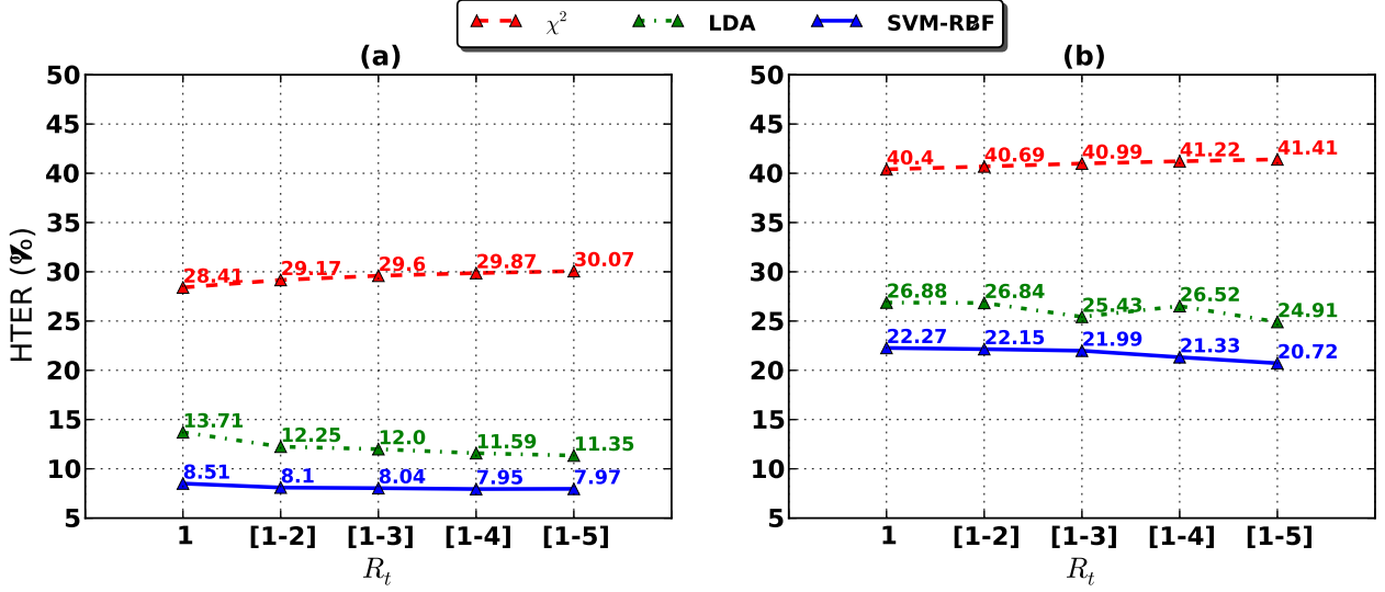
Figure 3.8: HTER(%) evaluation with \text{LBP-TOP}_{8,8,8,1,1,R_t}^{u2} using different classifiers (a) Replay Attack Database (b) CASIA FASD.
