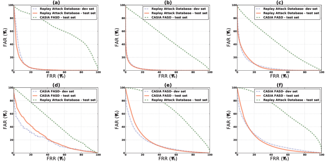
Figure 4.5: ROC curves of each countermeasure using the intra-test and the inter-test protocol. (a) Correlation with frame differences countermeasure trained and tuned with the Replay Attack Database (b) LBP-TOP countermeasure trained and tuned with the Replay Attack Database (c) LBP countermeasure trained and tuned with the Replay Attack Database (d) Correlation with frame differences countermeasure trained and tuned with the CASIA FASD (e) LBP-TOP countermeasure trained and tuned with the CASIA FASD (f) LBP countermeasure trained and tuned with the CASIA FASD.
