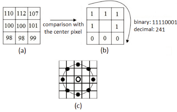
Figure 3.1: LBP operator. (a) and (b) The basic LBP operator, where the neighbourhood of each pixel is thresholded and a binary number is obtained. (c) A circular neighbourhood example (with 8 neighbour points and radius 2). The pixel values are bilinearly interpolated whenever the sampling point is not in the center of a pixel.
