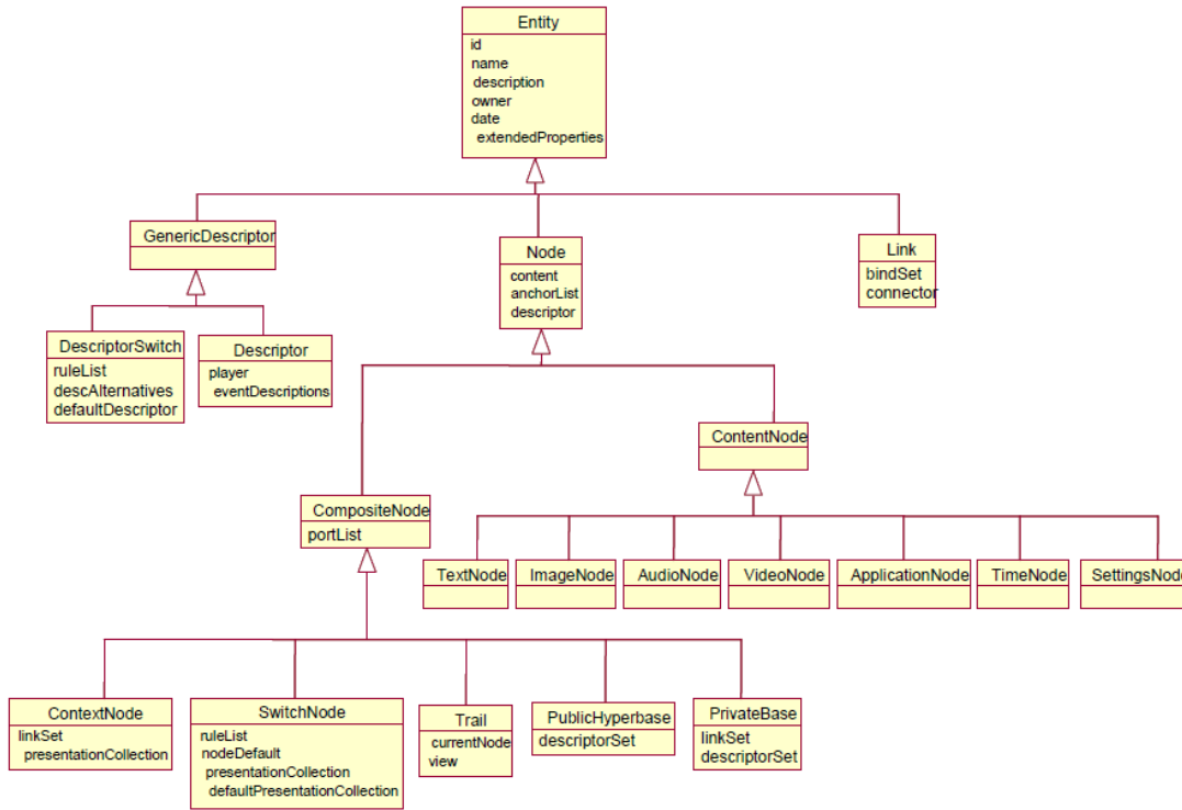
Figure 3.1: Overview of NCM class hierarchy [19]
