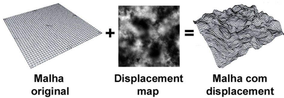
Fig. 3.5: Displacement mapping shader.
