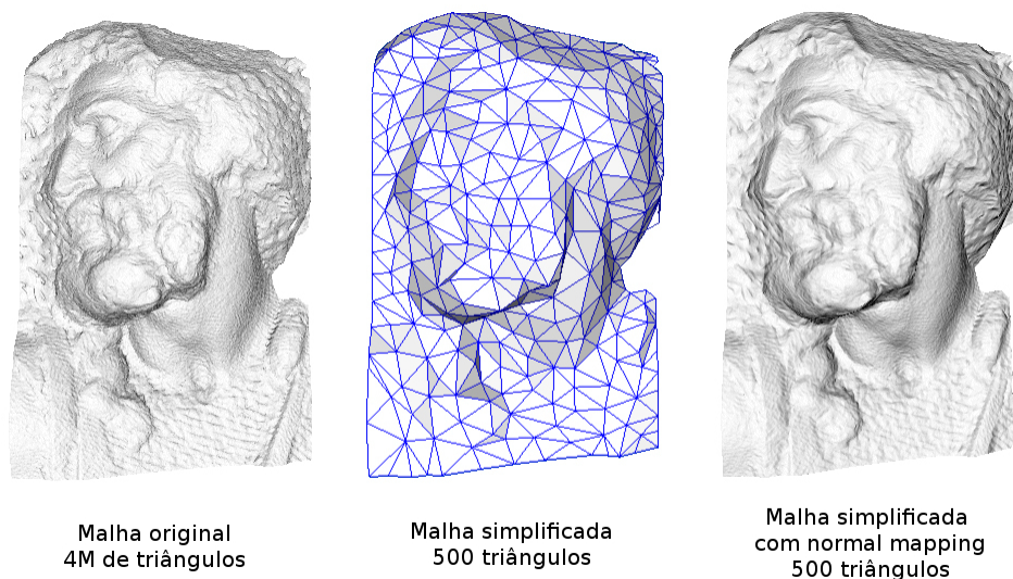
Fig. 3.9: Normal mapping.
