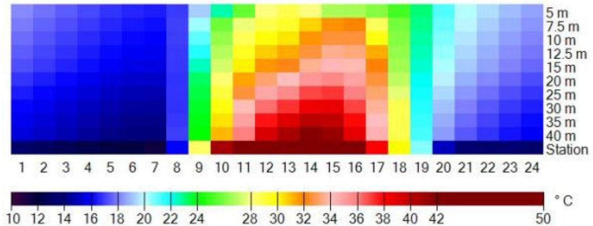
Fig 39 . Diurnal courses of Mean Radiant Temperature ( T_{mrt} ) ( ^{\circ}\text{C} ) for an urban canyon with east-west orientation.
