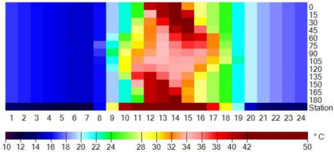
Fig 43. Diurnal courses of Mean Radiant Temperature ( T_{mrt} ) (°C) for the stepwise (15°) rotation of an urban canyon with a height and width of 15m based on data from climate station for the period June 25th, 2003 to December 31st, 2010.
