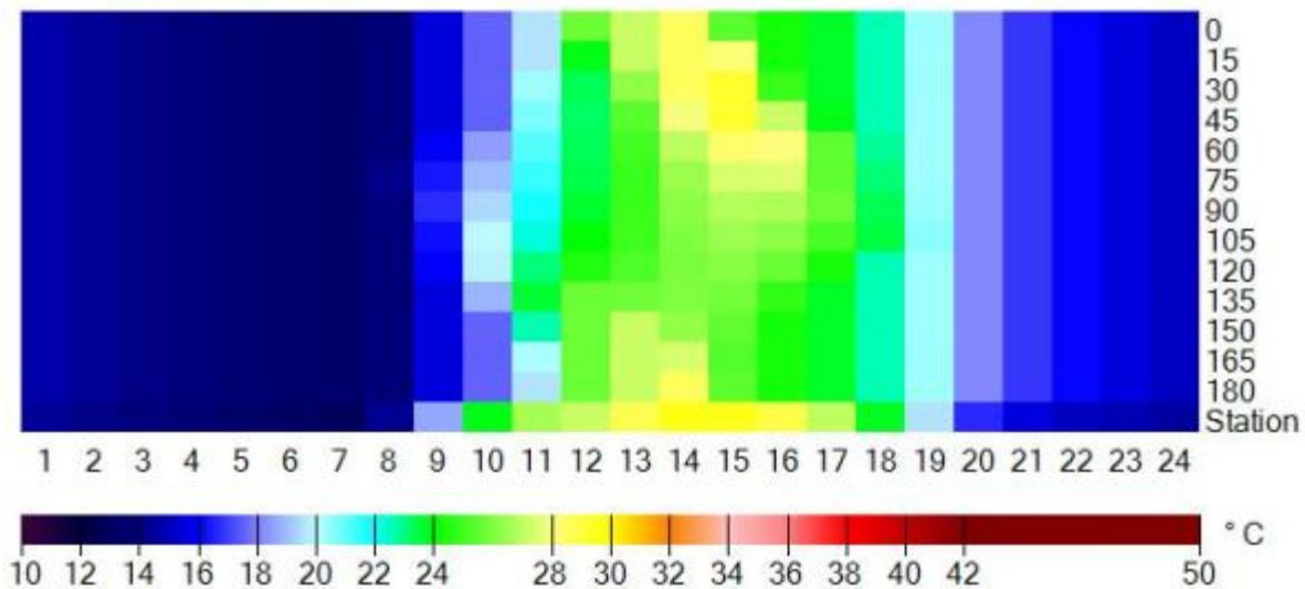
Fig 42. Diurnal courses of Physiologically Equivalent Temperature (PET) ( ^\circ\text{C} ) for the stepwise ( 15^\circ ) rotation of an urban canyon with a height and width of 15m based on data from climate station for the period June 25th, 2003 to December 31st, 2010.
