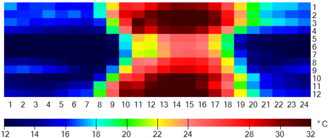
Fig 30. The mean monthly diurnal course of PET (°C) based on the data of the urban climate station and for the period June 25th, 2003 to December 31st, 2010.
