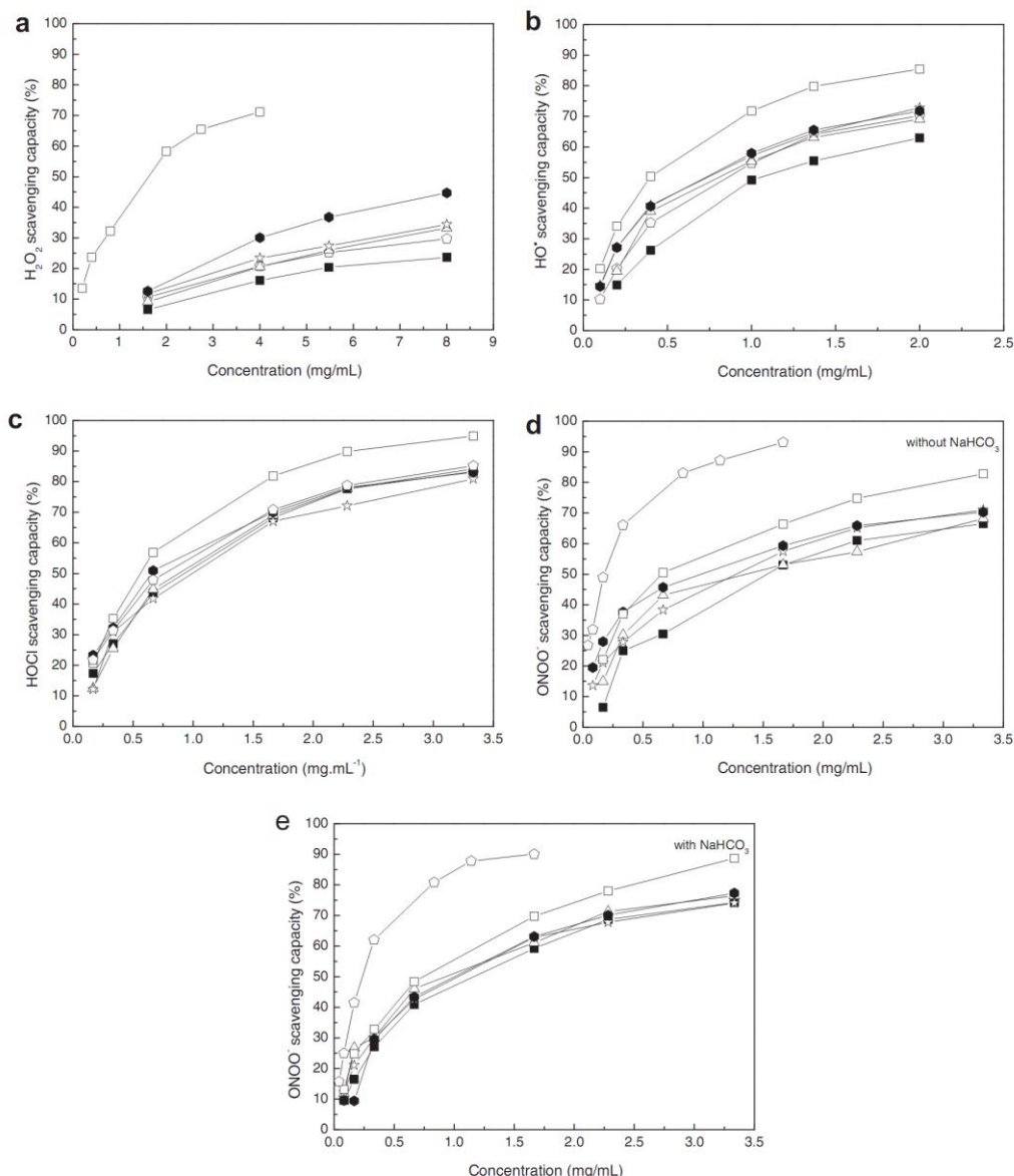
Fig. 2. Gum arabic microcapsules scavenging capacity of (a) hydrogen peroxide ( H_2O_2 ), (b) hydroxyl radical ( HO^\bullet ), (c) hypochlorous acid (HOCl), (d) anion peroxynitrite ( ONOO^- ) without NaHCO_3 and (e) ONOO^- with NaHCO_3 . Legend: filled square: empty microcapsule (no antioxidant molecule), open triangle: tocopherol microcapsule, open star: apo-12'-carotenal microcapsule, filled hexagon: apo-8'-carotenal microcapsule, open square: \beta -carotene microcapsule, open pentagon: trolox microcapsule.
