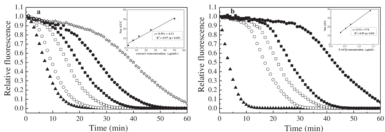
Fig. 6 Fluorescence decay of fluorescein induced by peroxy radicals in the presence of different concentrations of (a) phenolic extract and (b) 5-caffeoylquinic acid standard. Legend (a): blank (filled triangle), 1.25 \mu\text{g/mL} (open circle), 6.25 \mu\text{g/mL} (open square), 12.5 \mu\text{g/mL} (filled square), 25.0 \mu\text{g/mL} (filled circle) and 50.0 \mu\text{g/mL} (open star). Legend (b) blank (filled triangle), 0.35 \mu\text{g/mL} (open circle), 0.53 \mu\text{g/mL} (open square), 0.70 \mu\text{g/mL} (filled square) and 1.40 \mu\text{g/mL} (filled circle). Inset: linear relationship between (a) phenolic extract and (b) 5-caffeoylquinic acid concentrations and net AUC values from the fluorescence decay curves of fluorescein oxidation.
