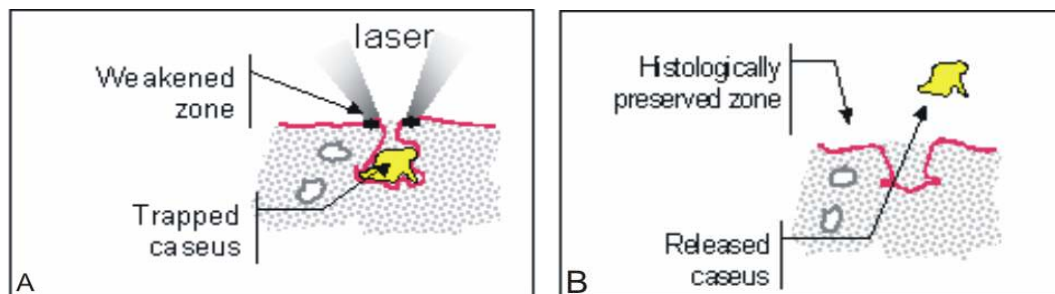
Figures 6A and 6B- Schematic representation of CO_2 LCC procedure. A) Low-energy density is applied around the crypt, causing an immediate weakening zone hit by the laser beam. B) CO_2 laser caused the widening of the opening ostium and shallowing of the crypt, resulting in elimination of debris and of other residues, facilitating and preventing caseum retention.
