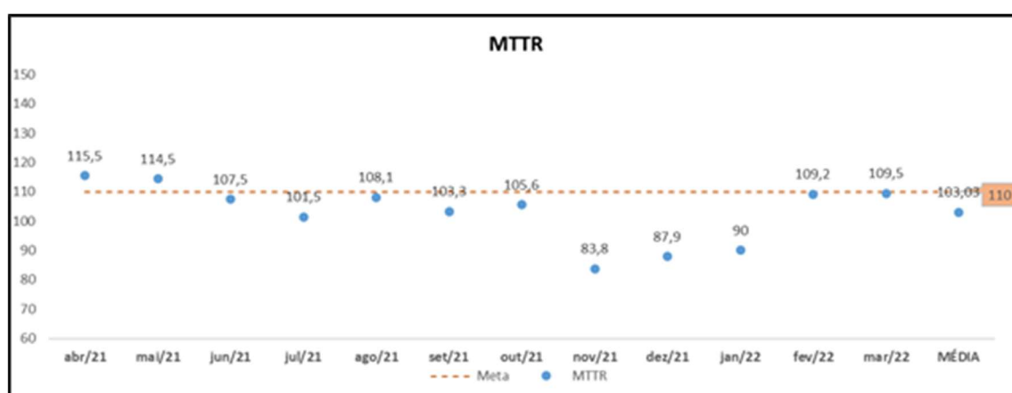
Figura 7 - Indicador MTTR ( Mean Time to Repair ).
